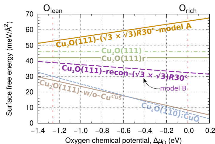
Figure A1. Surface energies of Önstén's models A and B of the (\sqrt{3} \times \sqrt{3})R30^\circ reconstructed \text{Cu}_2\text{O}(111) surface—the difference between the two models is that model A contains \text{Cu}^{\text{CUS}} ions—compared to surface energies of other surfaces, which are shown as faded. Notice that the model A is predicted to be the least stable among the considered surface models, which is in agreement with GGA+U calculations of Bendavid and Carter [24].
