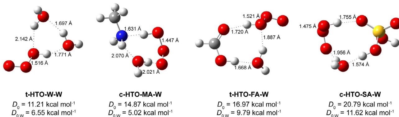
Figure 3: Optimised structures of the most stable t-HTO-W-W, c-HTO-MA-W, t-HTO-FA-W and c-HTO-SA-W complexes with the B3LYP/6-311++G(3df,3pd) bond lengths and the CBS-QB3 binding energies. Dotted lines represent intermolecularly formed H-bonds.
