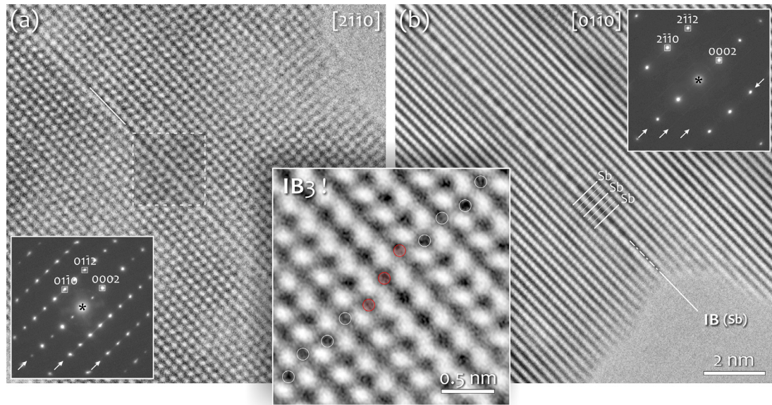
Fig. 7. HRTEM study of IBs in \text{Sb}_2\text{O}_3 -doped ZnO in two low-index crystallographic projections: (a) [2\bar{1}10] and (b) [01\bar{1}0] , with the corresponding electron diffraction patterns. IBs are characterized by lateral expansion due to the inversion of polarity. Black dots in HRTEM images correspond to cation columns, allowing to track the stacking sequence in (a), and cation ordering in (b). Close-up of HRTEM image in the [2\bar{1}10] projection clearly shows a stacking configuration with a single ccp sequence (red circles) across the IB plane ( \text{IB}_3 ). (For interpretation of the references to color in this figure legend, the reader is referred to the web version of this article.)
