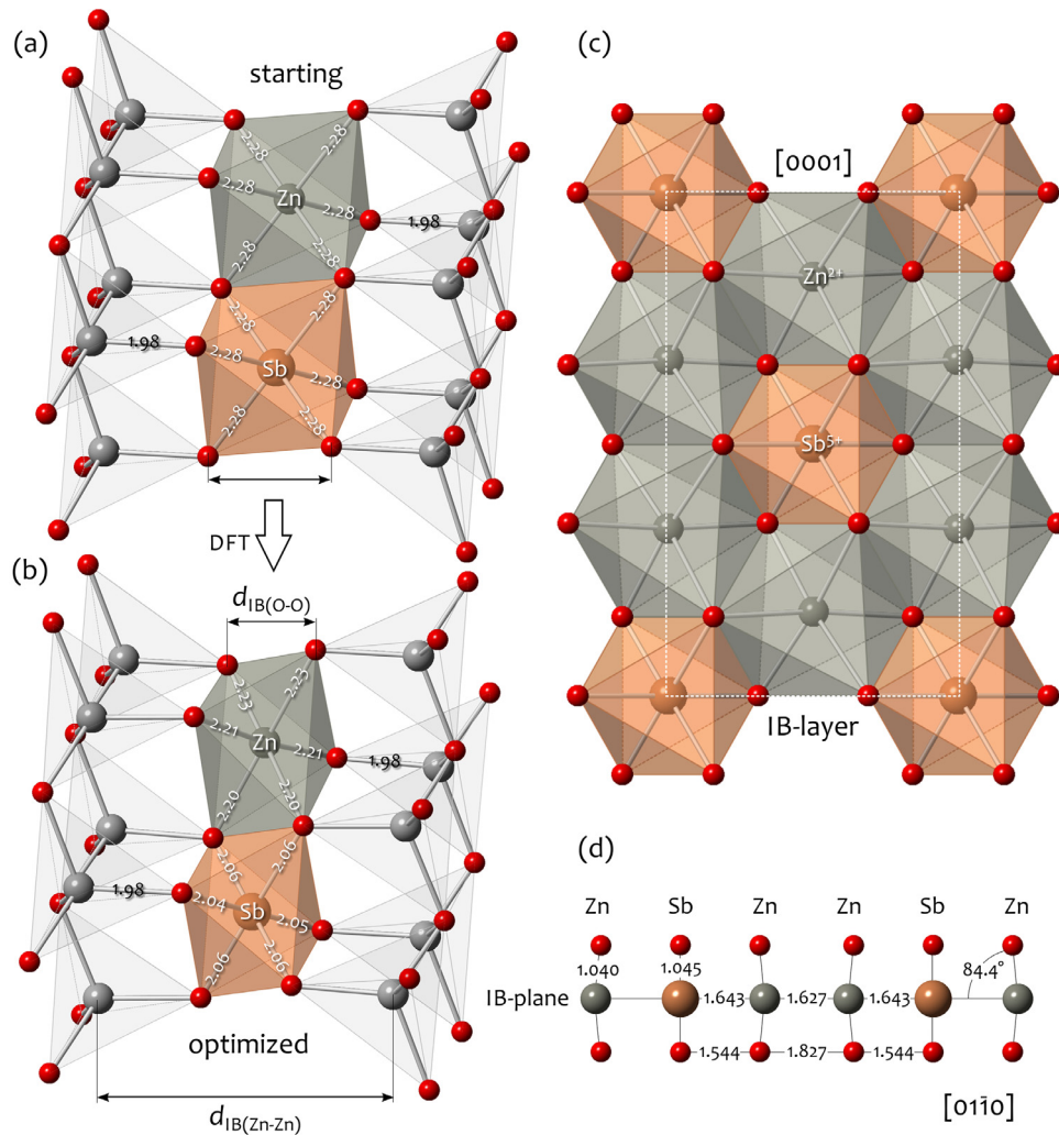
Fig. 6. Bond lengths in the IB layer (a) before and (b) after DFT relaxation resulting in a lateral contraction of the bulk parts. IB characteristic distances d_{IB(O-O)} and d_{IB(Zn-Zn)} defining IB-octahedra width and the distance between the Zn-planes in adjacent domains, respectively. (c) IB-layer in [0001]-projection showing a honeycomb distribution of cations ( Zn^{2+} and Sb^{3+} ). The Sb–O bond lengths are 10% shorter than the corresponding Zn–O bond lengths. (d) Undulation of projected bond lengths and torsion angles in IB-plane viewed in [0110].
