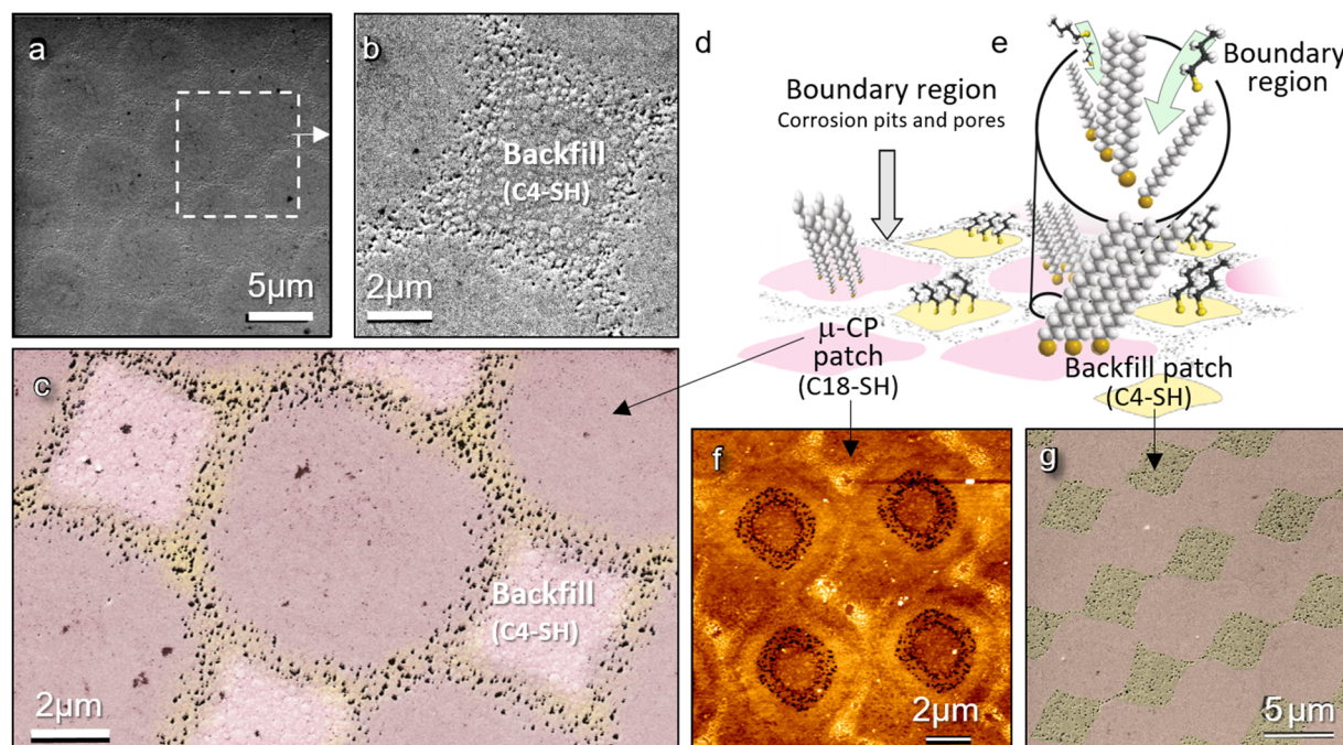
Fig. 4 Localized initial dealloying along artificial SAM patch boundaries. a SEM image of \mu\text{CP-C}_{18}\text{-SH}/\text{C}_4\text{-SH} modified type-A surface after dealloying. b Zoom-in to initial dealloying region, contrast-enhanced SEM image. c Color-modified SEM image showing localized initial dealloying along artificial SAM boundaries. d Illustration representing initially localized dealloying, with (e) highlighting of the interface region. f Occasionally observed double-ring pit area, AFM image. g SEM image, localized dealloying is restricted to \text{C}_4\text{-SH} patches after additional cycles.
