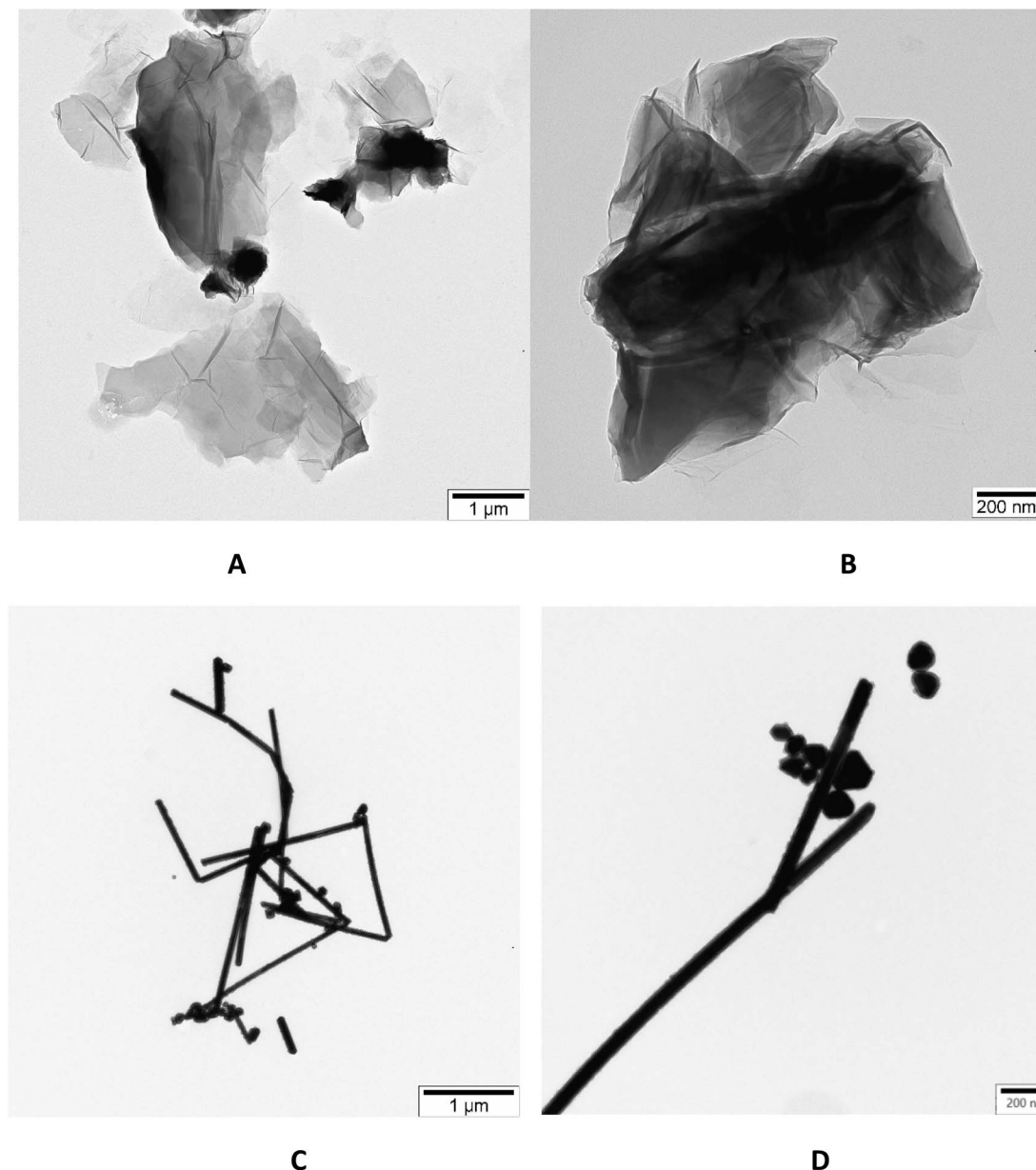
Fig. 4 TEM images of nanomaterials: (A and B) GO nanosheets, (C and D) Ag nanowires.
