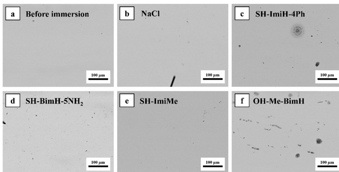
Fig. 16. SEM images of \text{Cu}_{40}\text{Zr}_{60} amorphous alloy (a) prior to immersion and after 120 h immersion in (b) 3 wt% NaCl with added (c) SH-ImiH-4Ph, (d) SH-BimH-5 \text{NH}_2 , (e) SH-ImiMe, and (f) OH-Me-BimH.
