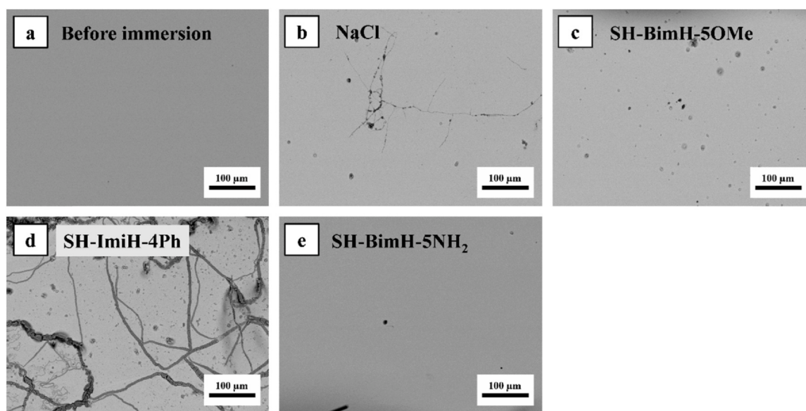
Fig. 17. SEM images of \text{Cu}_{50}\text{Zr}_{50} amorphous alloy (a) prior to immersion and after 120 h immersion in (b) 3 wt% NaCl, and with added (c) SH-BimH-5OMe, (d) SH-ImiH-4Ph, and (e) SH-BimH-5 \text{NH}_2 .
