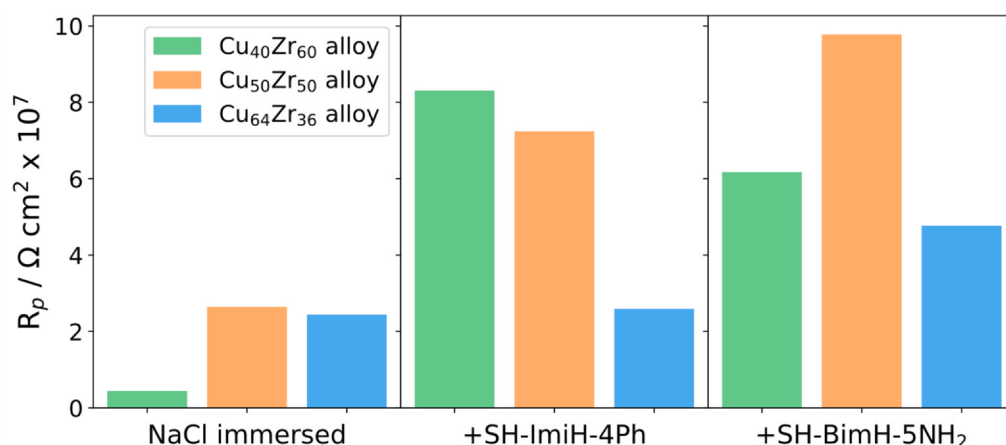
Fig. 14. Polarization resistance ( R_p ) of \text{Cu}_{40}\text{Zr}_{60} , \text{Cu}_{50}\text{Zr}_{50} and \text{Cu}_{64}\text{Zr}_{36} amorphous alloys with and without added 1 mM inhibitor compounds (either SH-ImiH-4Ph or SH-BimH-5NH 2 ) in 3 wt% NaCl solution.
