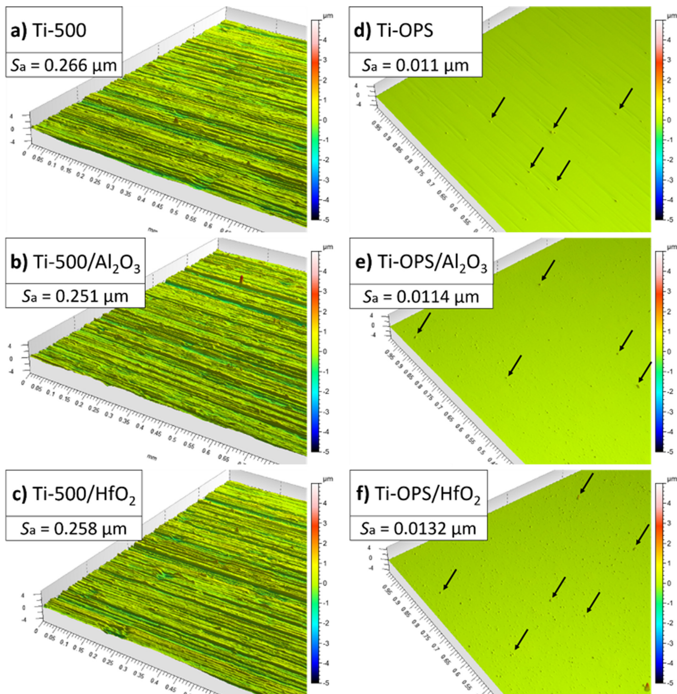
Fig. 1. 3D surface profiles of differently prepared bare and coated specimens of cp-Ti and their roughness values ( S_a ) obtained by profilometry, a) bare ground cp-Ti surface; b) ground cp-Ti surface coated with alumina; c) ground cp-Ti surface coated with hafnia; d) bare, polished cp-Ti surface; e) polished cp-Ti surface coated with alumina; f) polished cp-Ti surface coated with hafnia. Arrows in polished specimens denote the spots from which the \text{SiO}_2 particles were removed.
