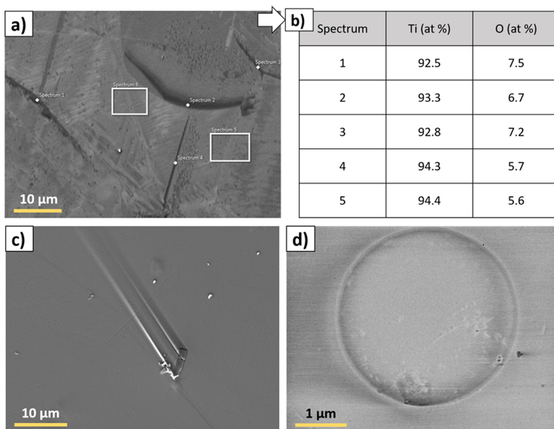
Fig. 3. a) SEM image of polished cp-Ti surface, recorded using the back-scattered electrons (LBE detector), magnification was 2000 ×, and b) chemical composition determined by EDXS analysis on numerated spots in SEM image in a). SEM images showing the morphology of c) embedded SiC particles in the Ti-OPS surface coated with alumina, recorded using the secondary electrons (LEI detector); magnification was 2300 ×, and d) of the site of the removed SiO 2 particle, recorded using the secondary electrons (SEI detector); magnification was 22,000 ×. The beam acceleration voltage was 5 kV for all presented images.
