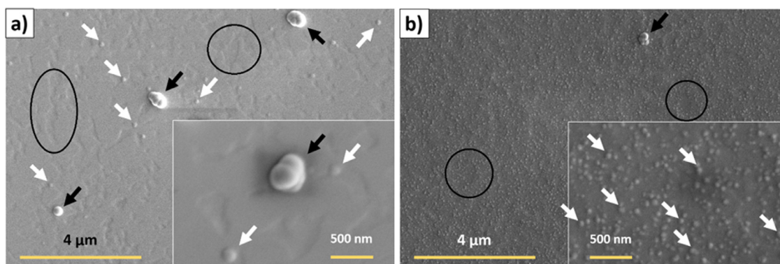
Fig. 4. SEM images recorded using secondary electrons (standard ETD detector), of a) alumina and b) hafnia thin films deposited on the Ti-OPS surface. Magnification was 10,000 × and 50,000 × (insets) and beam acceleration voltage 2 kV. White arrows denote ALD agglomerates or crystallites, black arrows denote larger contaminant particles, and black circles denote irregular features grown on oxygen-rich sites of the substrate (Fig. 3a,b).
