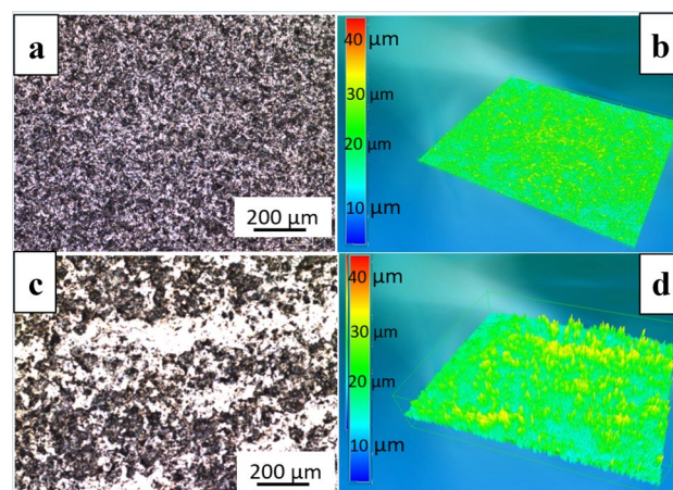
Fig. 4 Typical a, c 2D and b, d 3D images of unworn and worn areas on retrieved Alivium femoral heads. The difference in surface roughness is evident in 2D images; in 3D images, the colour scale defines the magnitude of roughness
