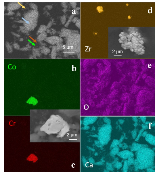
Fig. 7 Morphology and composition of wear particles isolated from periprosthetic tissue by alkaline protocol. a SEM BSE image showing particles differing in composition (heavy elements appear darker than bright ones), as pointed out by arrows. B–f EDS compositional maps of the SEM image in Co, Cr, Zr, O, and Ca. Arrows of the same colour note the presence of particles in the SEM image in ( a ). SEM BSE image of the metal particle is shown in the inset in ( c ). SEM BSE image of \text{ZrO}_2 particles added to polymethylmethacrylate bone cement is shown in the inset in ( d )
