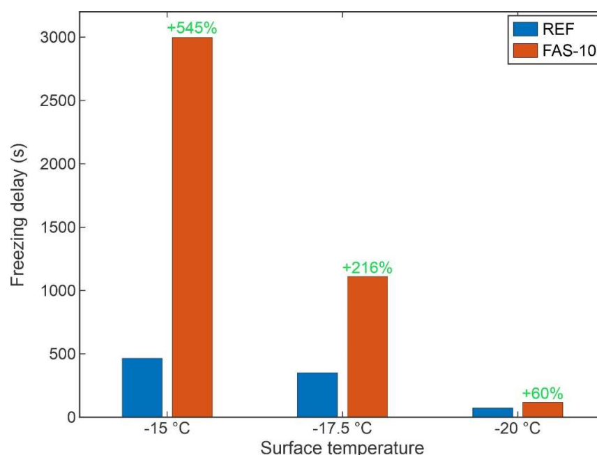
Figure 10. Freezing delay on the untreated reference surface (REF) and on the superhydrophobic etched FAS-10 surface at three surface temperatures. The relative enhancement is provided in green text.
