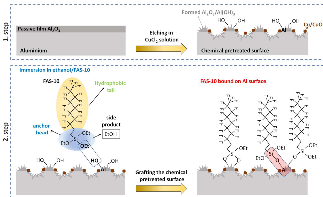
Figure 1. The schematic presentation of a two-step process to form a (super)hydrophobic aluminium surface. Firstly, the aluminium surface undergoes a chemical etching process in a \text{CuCl}_2 solution (1. step), followed by the second step of grafting the surface with perfluoroalkyl silane, FAS-10 (2. step).
