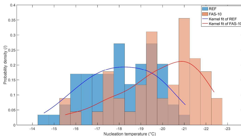
Figure 9. Probability density histograms and Kernel fits of the ice nucleation temperature on the untreated reference surface (REF) and on the superhydrophobic etched FAS-10 surface. Brown colour represents overlapping between blue and other colours.
