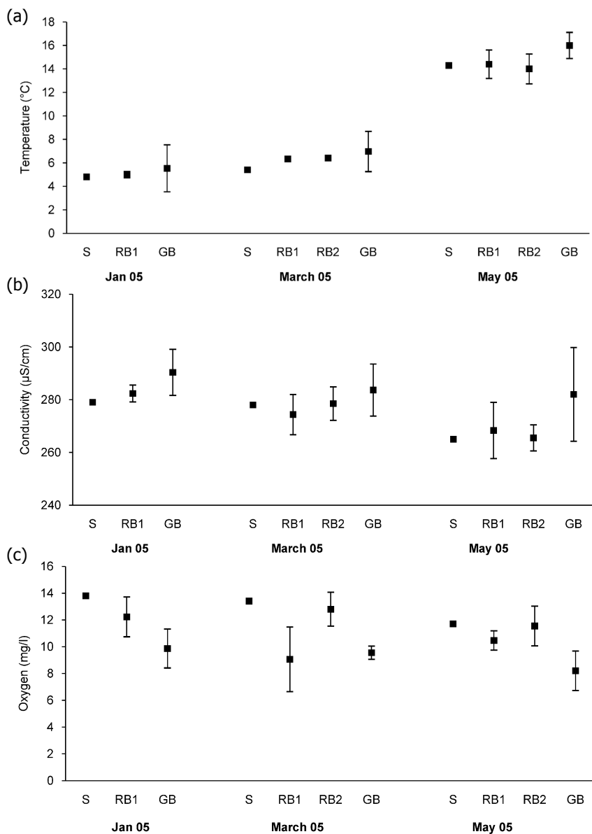
Figure 2. Mean temperatures (a) , conductivity (b) and oxygen concentrations (c) ( \pm SE) of surface and hyporheic water measured during invertebrate sampling. RB1 – shallow hyporheic zone (30 – 60 cm); RB2 – deeper hyporheic zone (60 – 90 cm); GB – gravel bars (60 – 90 cm). RB1, GB, n=3 ; RB2, n=2 .
