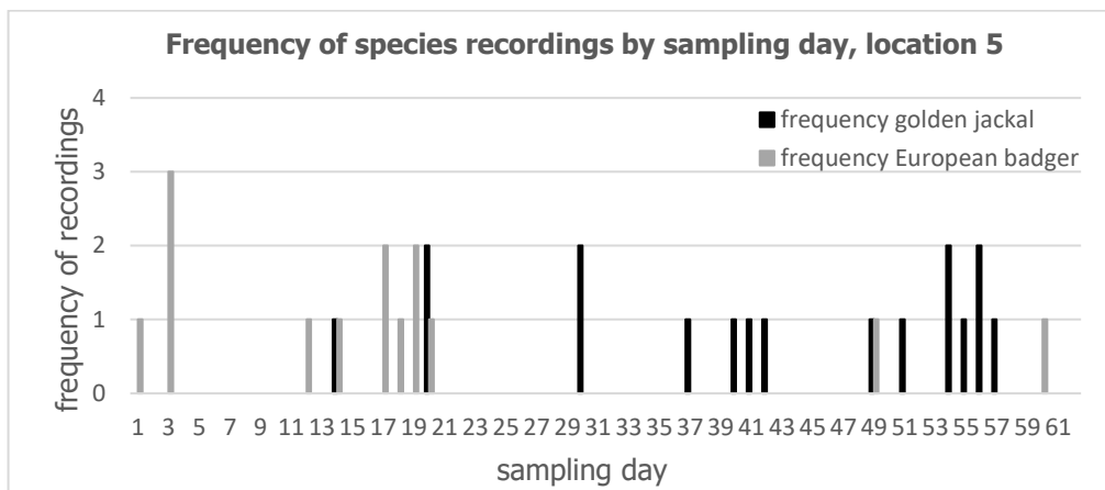
Figure 3. The frequency of jackal and badger recordings by sampling days (sampling from 26 March to 27. 5. 2022) at site five. The graph clearly indicates that at around the same time when the frequency of badger recordings drops, the frequency of jackal recordings increases.
