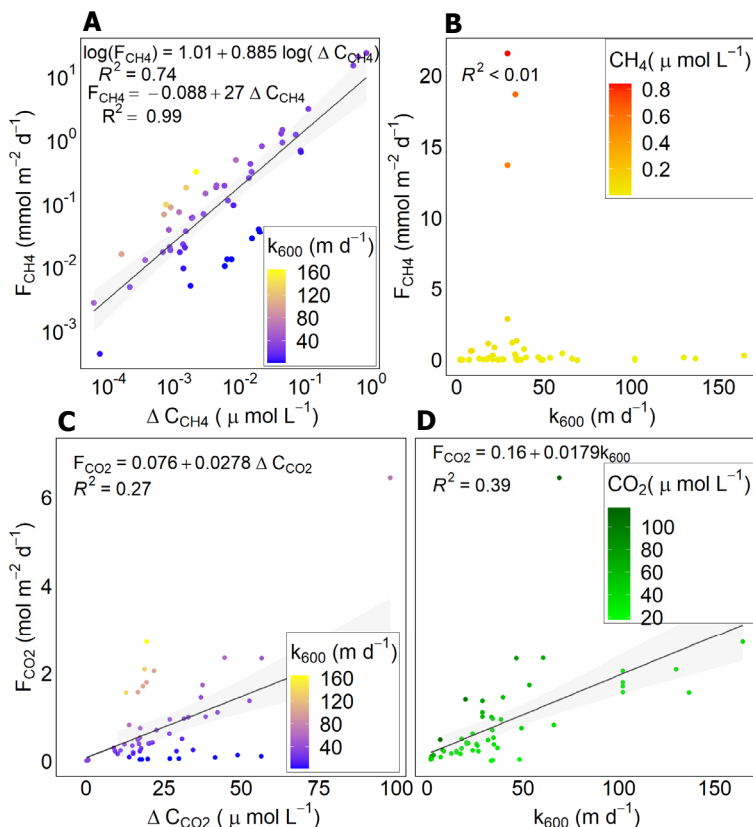
Figure 6. Relationship between CH 4 evasion rate (in mmol m -2 d -1 ) to \Delta C_{CH_4} (A) and to k_{600} (B) and between CO 2 evasion rate (in mol m -2 d -1 ) to \Delta C_{CO_2} (C) and to k_{600} (D) in a simple linear regression. \Delta C is computed as the difference between dissolved and atmospheric concentration. The black lines represent a linear regression with the gray area showing 95% confidence intervals for the linear model. Fitting parameters are found in the model equation of respective plots. Note: the axes of plot A have a logarithmic scale and model equations for F_{CH_4} as function of C_{CH_4} are given for log-transformed and non-log transformed values.
