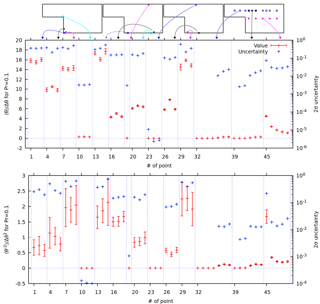
Figure 14. x-axis: number of point according to Figure 2. Top: Mean temperature for Pr = 0.1 . Bottom: \theta_{RMS} for Pr = 0.1 . Red dots represent root-mean-square values with \pm 2\sigma range (left scale), blue dots represent (2\sigma) uncertainty (right scale).
