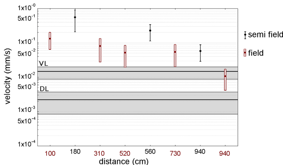
Figure 2. Maximum (mean \pm SD) substrate velocity (mm/s, logarithmic scale) of disruptive signal (DN) recorded in the frequency range 50-300 Hz from potted plants in semi-field conditions and from rooted grapevine plants in field. Semi-field and field recordings were made at three and five distances from a DN source, respectively (semi-field: black dots, distances 180 cm, 560 cm, 940 m; field: red dots, distances 100 cm, 310 cm, 520 cm, 730 cm, 940 cm). MCS played back into potted plants from a leaf showed highest substrate velocities within the same vibrated leaf (VL) range; a substantial decrease was found on all other leaves of the plant (distant leaves, DL). The transverse black lines represent the mean ( \pm SD, gray areas) of maximum velocity of MCS of the VL or DL range. doi:10.1371/journal.pone.0032954.g002
