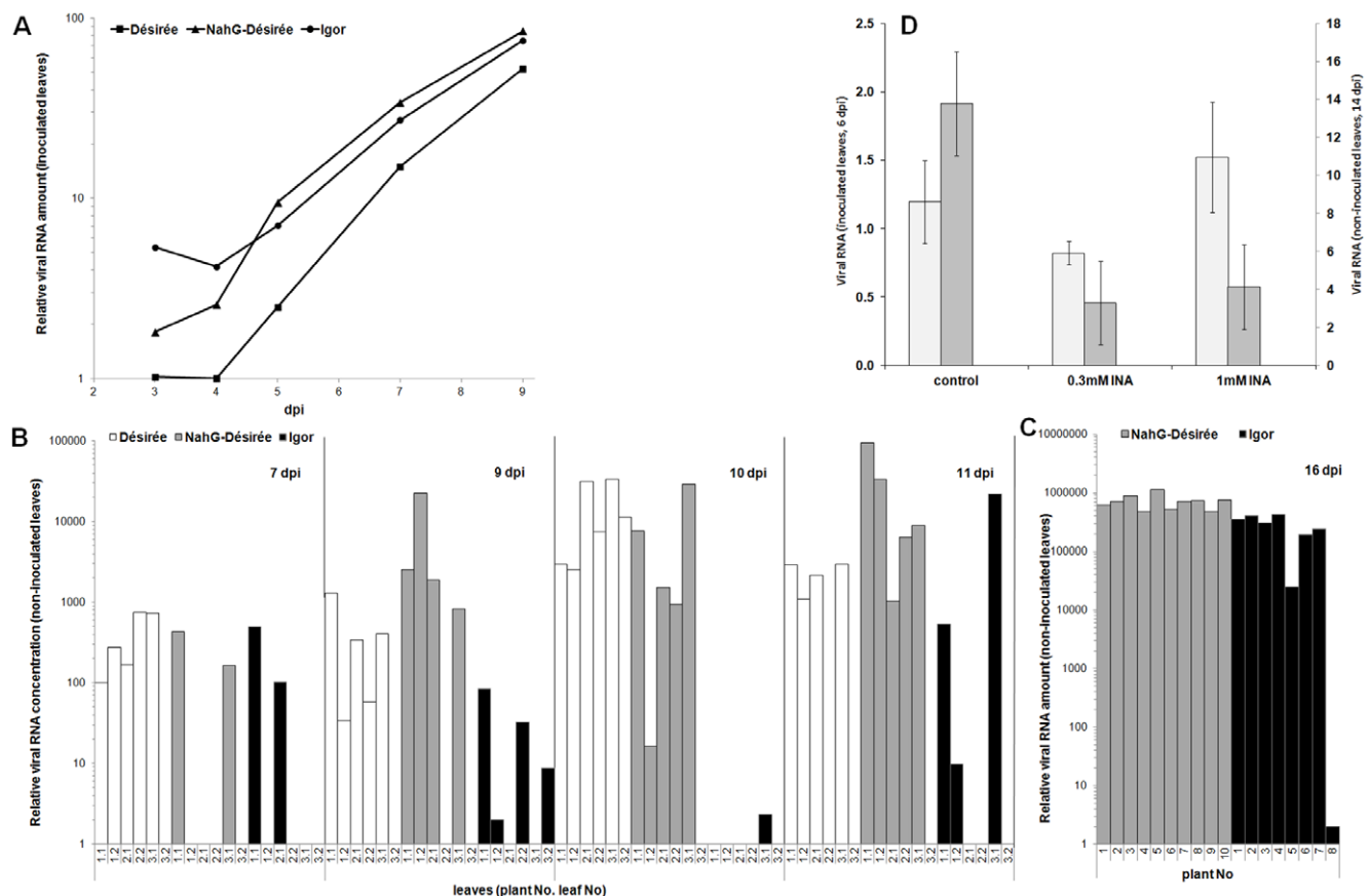
Figure 2. Accumulation of PVY RNA in leaves of potato plants. (A) Relative PVY RNA concentration (average of 3 individual plants) in inoculated leaves 3–9 days post inoculation (dpi). Results of statistical evaluation of data are shown in Table 1 . (B) PVY RNA concentration (relative to the lowest detected viral amount) in non-inoculated leaves (3 plants per genotype, 2 leaves per plant: e.g. 1.2 denotes second leaf of plant 1) 7–11 dpi. (C) PVY RNA concentration in non-inoculated leaves of ten NahG-Désirée and eight cv. Igor plants at 16 dpi. PVY RNA concentrations are presented relative to the lowest detected viral amount in all plants. (D) Relative PVY RNA concentration ( \pm SE, n=4 , normalised to COX gene expression) in the inoculated leaves 6 dpi (light grey) and in non-inoculated leaves 14 dpi (dark grey) of the NahG-Désirée plants following treatment with water (control), 0.3 mM or 1 mM INA. doi:10.1371/journal.pone.0029009.g002
