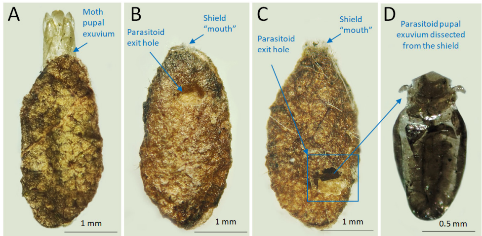
Figure 5. Abandoned shields of C. lucifluella . A – the shield with moth pupal exuvium protruding from the shield “mouth”; B , C – the shields with parasitoid exit hole; D – the pupal exuvium of an eulophid dissected from the shield. A – Sochi, B–D – Abkhazia, 2023. Photos: N. Kirichenko.
