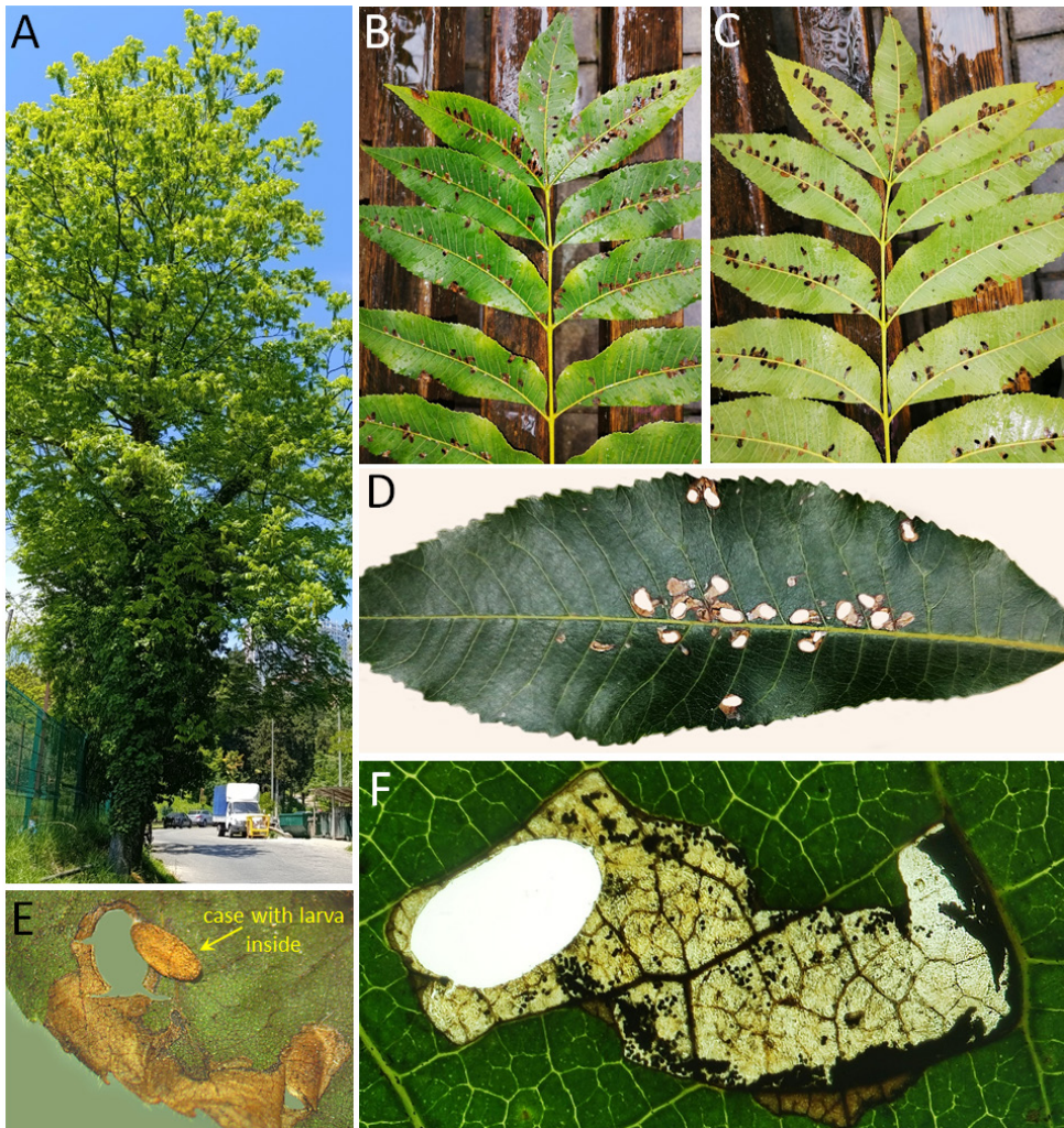
Figure 3. The damage caused by C. lucifluella in Sochi (Russia) in 2023. A – a tree of Car. il-linoensis in the city planting; B, C – a compound leaf with numerous mines, upper side ( B ) and lower side ( C ) views; D – an individual compound leaf with the vacated mines along the main vein; E – a shield with a larva inside cut from leaf mine; F – the vacated leaf mine with an oval hole remained after larva cut out the shield. Photo: E. Shoshina ( A ), E. Zhuravleva ( B, C, E ), N. Karpun ( D ), N. Kirichenko ( F ).
