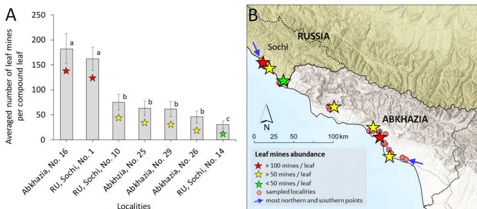
Figure 4. Averaged number of C. lucifluella 's mines ( \pm SD) on compound leaves of Car. illinoensis in Sochi (Russia, RU) and Abkhazia. The columns with different letters are statistically distinct (Mann-Whitney U-test, p < 0.05 ). The sampled localities (Nos 1, 10, 14, 16, 26, 29) are coded in figure A, and indicated by the stars in figures A, B. The stars of different colors reflect leaf mine abundance (per compound leaf). Sampled localities are provided in Fig. 1.
