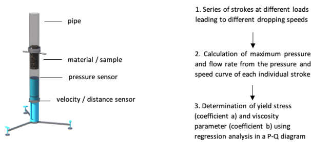
Figure 5. Sliper setup and measurement procedure [51].
