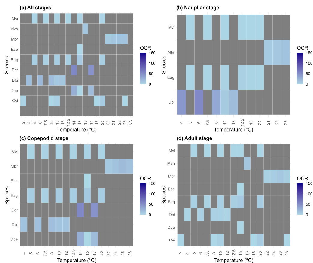
Figure 3. A heatmap of oxygen consumption rates (OCRs; \mu\text{L O}_2/\text{mg DW} \times \text{h} ) of freshwater cyclopoid species across a temperature gradient: (a) all stages; (b) nauplii; (c) copepodids; (d) adults. Colour intensity indicates OCR magnitude. Mvi: Megacyclops viridis (Jurine, 1820); Mbr: Mesocyclops brasiliensis Kiefer, 1933; Ese: Eucyclops serrulatus serrulatus (Fischer, 1851); Eag: Eucyclops agilis agilis (Koch, 1838); Dcr: Diacyclops crassicaudis crassicaudis (Sars G.O., 1863); Dbi: Diacyclops bicuspidatus bicuspidatus (Claus, 1857); Mva: Microcyclops varicans varicans (Sars G.O., 1863); Cvi: Cyclops vicinus vicinus Uljanin, 1875; Dbe: Diacyclops belgicus Kiefer, 1936.
