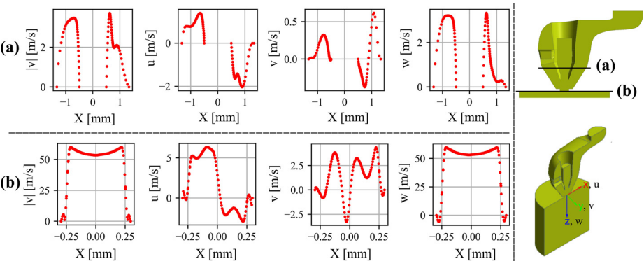
Figure 8. Velocity profiles of magnitude |v| and u , v , and w components for mesh D at (a) 1.3 mm inside the nozzle and (b) nozzle outlet
