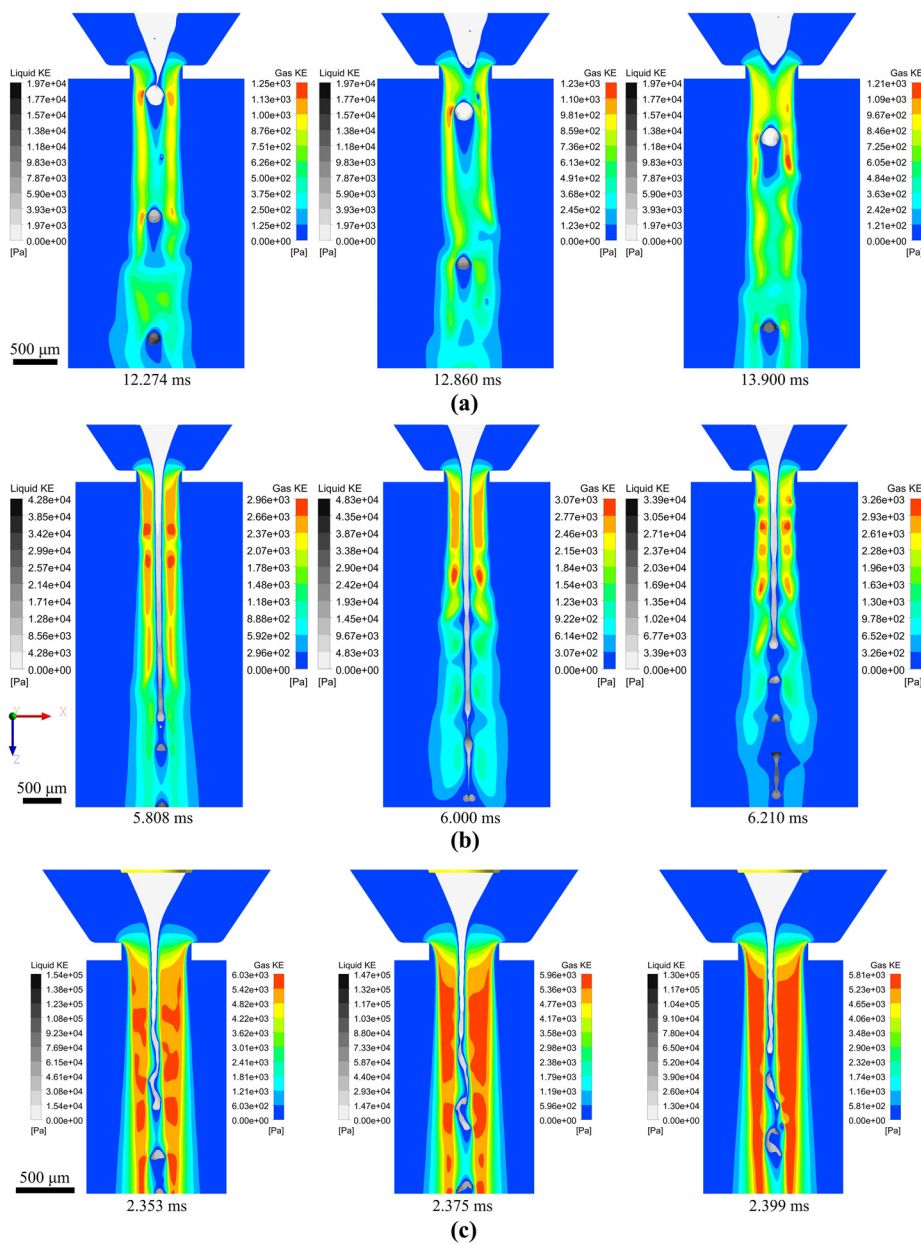
Figure 13. Specific kinetic energy of air and water for (a) dripping G25L500; (b) jetting G40L1000 and (c) whipping G60L1000 regime
