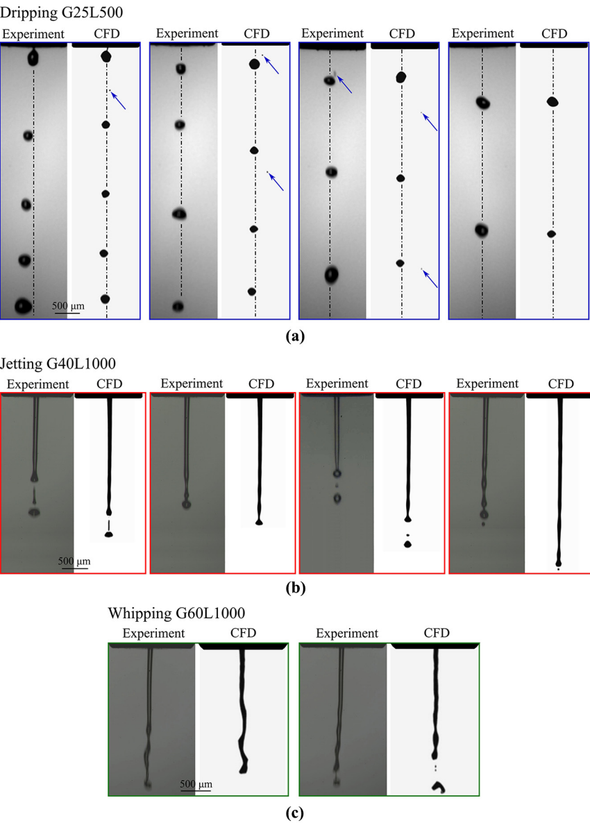
Figure 10. A comparison of experimental vs numerical jet shapes for (a) dripping G25L500; (b) jetting G40L1000 and (c) whipping G60L1000
