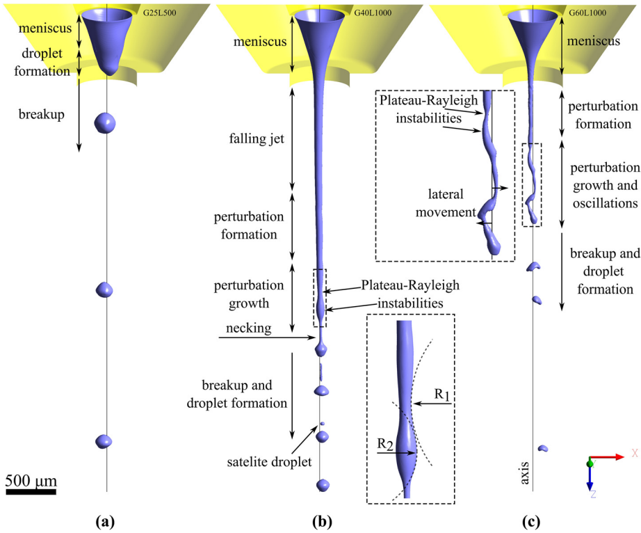
Figure 9. Isosurface of volume fraction of 0.5 for (a) dripping; (b) jetting and (c) whipping regime
