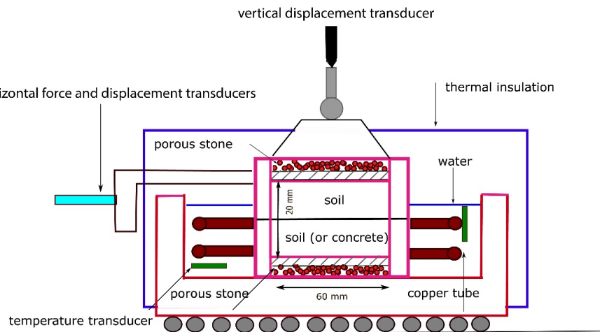
Figure 27. Direct shear apparatus with temperature control system (adapted from Reference [184]).
