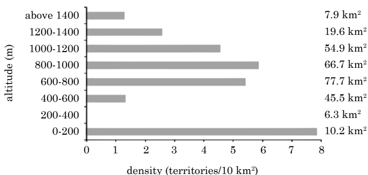
Fig. 2 - Density changing of the Ural Owl, Strix uralensis , according to the altitudinal distribution; survey areas sizes are shown at each altitudinal belt (joint data of systematic owl surveys; N_{\text{areas}} = 15 , N_{\text{survey points}} = 368 , N_{\text{owl territories}} = 126 ).
