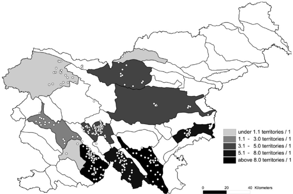
Fig. 1 - Distribution of the Ural Owl Strix uralensis in Slovenia with marked density estimations for better-searched regions.
