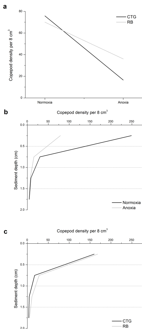
Fig. 6. First-order interactions of three-way ANOVA for factors (a) oxygen X method, (b) oxygen X depth and (c) depth X method. The geomean of copepod abundance is given. For each graph, the third factor (that is not shown) was averaged.
