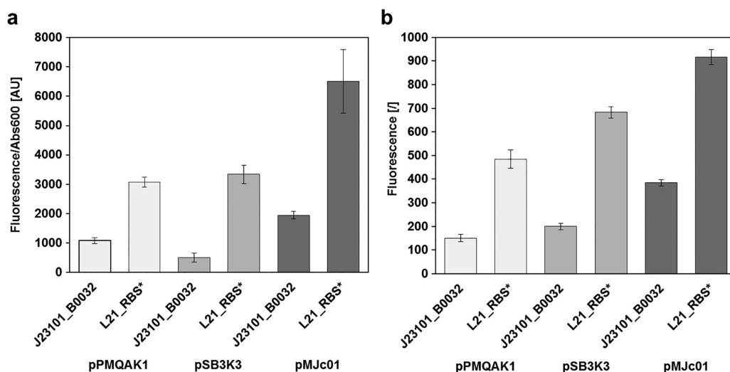
Figure 3 Relative GFPmut3b reporter expression from different plasmid backbones. GFPmut3b fluorescence intensity in E. coli transformed with pMJc01, pSB3K3, or pPMQAK1 containing different regulatory sequences in the reporter expression device. Differences between mean values for triplicates of cells with expressed GFPmut3b and cells with empty vector \pm standard deviation are shown. (A) GFPmut3b fluorescence intensity in cell cultures of E. coli . (B) GFPmut3b fluorescence intensity in cell lysates of E. coli . Full-size DOI: 10.7717/peerj.12199/fig-3
