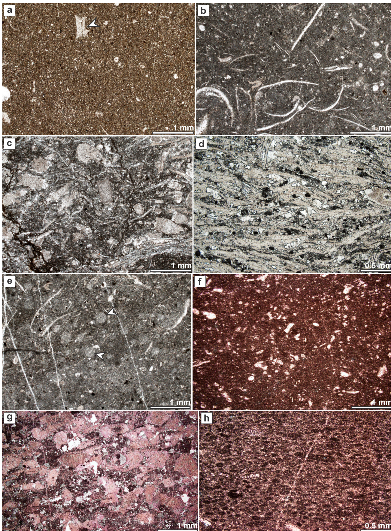
Fig. 16. Carbonate microfacies of the Ladinian – Carnian sedimentary succession of the Slovenian Basin (Pseudozilja and Amphiclina formations). a : Carbonate mudstone. Arrowhead points at the echinoderm. Sample Davča D1:23.3. b : Filament-echinoderm wackestone. Sample Hudajužna H19.5. c : Filament-echinoderm packstone. Sample Hudajužna H9.1. d : Filament packstone. Sample Zakojca ZK2:53. e : Radiolarian wackestone. Arrowheads point at calcified radiolarians. Note also the presence of filaments. Sample Hudajužna H36.2. f : Bioclastic wackestone. Sample Poče PO1:7. g : Crinoid packstone. Sample Zakojca ZK2:30. h : Peloid packstone. Sample Poče Po1:2.
