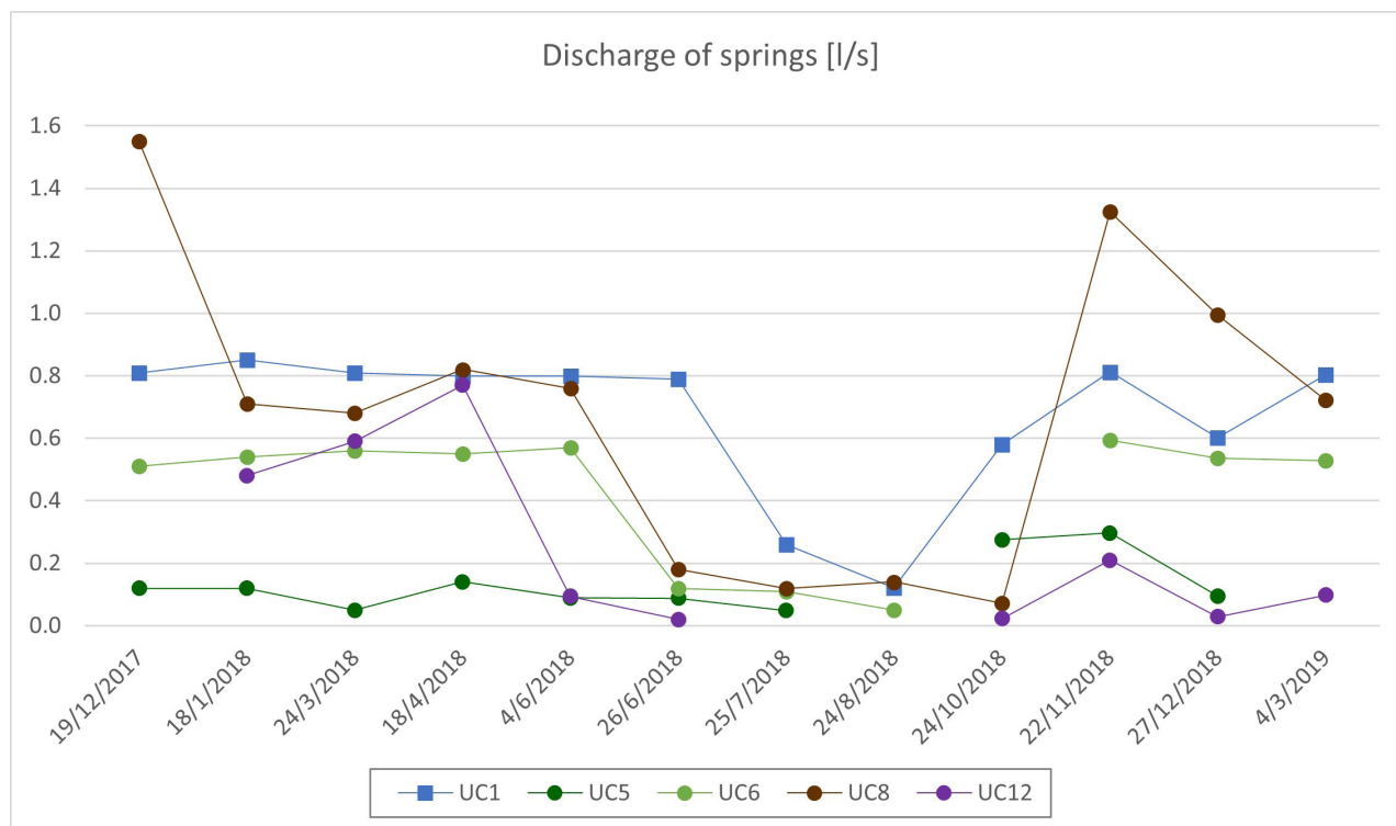
Fig. 5. Discharge of springs where taking of measurements was possible. Missing measurements are the result of the absence of spring water (springs were dry) at the time of sampling.
