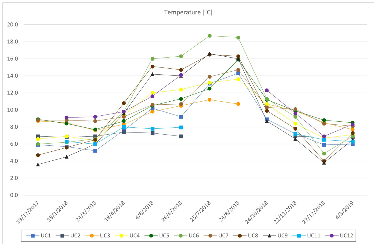
Fig. 6. Measured water temperatures (°C) at sampling sites in the Učja Valley.
