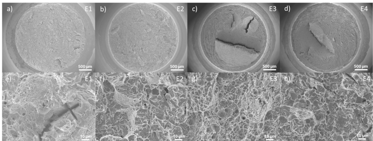
Fig. 3. (a, b, c, d) respective SEM photos of the entire fracture surfaces of specimens E1 to E4 tested in the air (magnification 33 \times ), and (e, f, g, h) fracture surfaces at the edge of the specimens (magnification 1000 \times ) for specimens E1 to E4, respectively.
