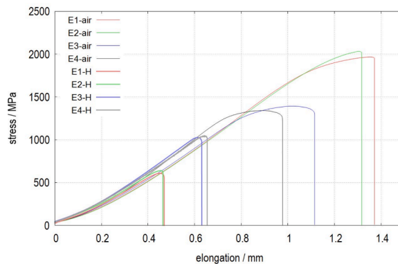
Fig. 2. Stress–elongation (displacement) curves for selected SSRT tests conducted in the air (thinner lines) and during hydrogen charging at a current density of 0.1 mA/cm 2 (thicker lines).
