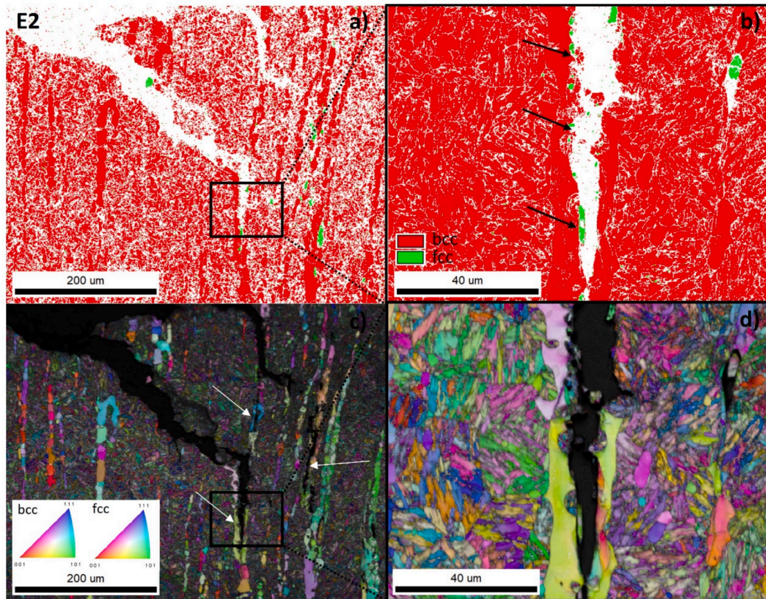
Fig. 7. EBSD phase maps of cracks in the axial plane of steel specimen E2, shown at different magnifications (a and b); bcc phase (red) – martensite and delta ferrite; fcc phase (green) – austenite; and the corresponding IPF + QI maps (c and d). The fracture is at the top. (For interpretation of the references to colour in this figure legend, the reader is referred to the web version of this article.)
