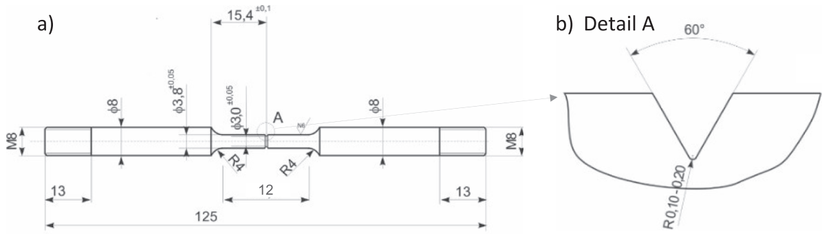
Fig. 1. Dimensions of the SSRT tensile specimen (a) with a V-notch (b).
