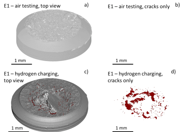
Fig. 5. MicroCT scans imaging the upper surface of the fractured end of the E1 specimen tested a) in the air and c) during hydrogen charging, with a visualization of the cracks (marked in red) for the same specimen tested b) in the air (no propagation of secondary cracks observed) and d) during hydrogen charging. (For interpretation of the references to colour in this figure legend, the reader is referred to the web version of this article.)
