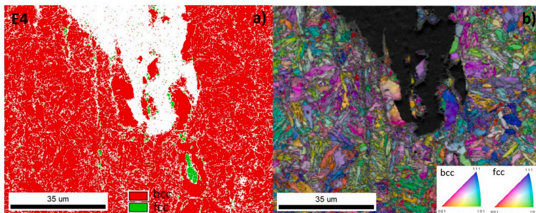
Fig. 9. (a) EBSD phase maps of the axial plane in the E4 specimen, containing the phases bcc (red) – martensite and delta ferrite and fcc (green) – austenite, and (b) the corresponding IPF + QI maps. The fracture is at the top. (For interpretation of the references to colour in this figure legend, the reader is referred to the web version of this article.)
