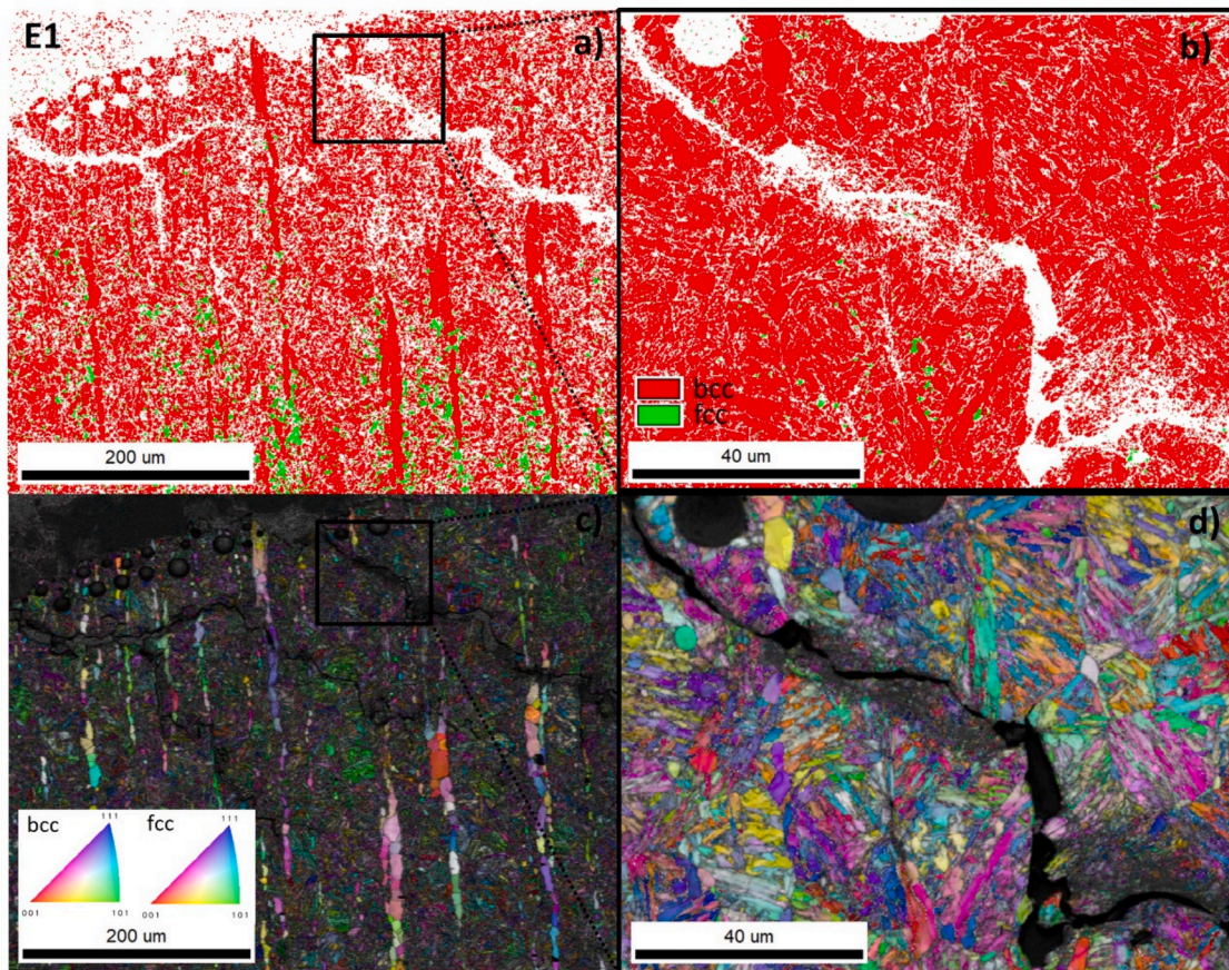
Fig. 6. EBSD phase maps of cracks in the axial plane of steel specimen E1, shown at different magnifications (a and b); bcc phase (red) – martensite and delta ferrite; fcc phase (green) – austenite; and the corresponding IPF + QI maps (c and d). The fracture is at the top. (For interpretation of the references to colour in this figure legend, the reader is referred to the web version of this article.)
