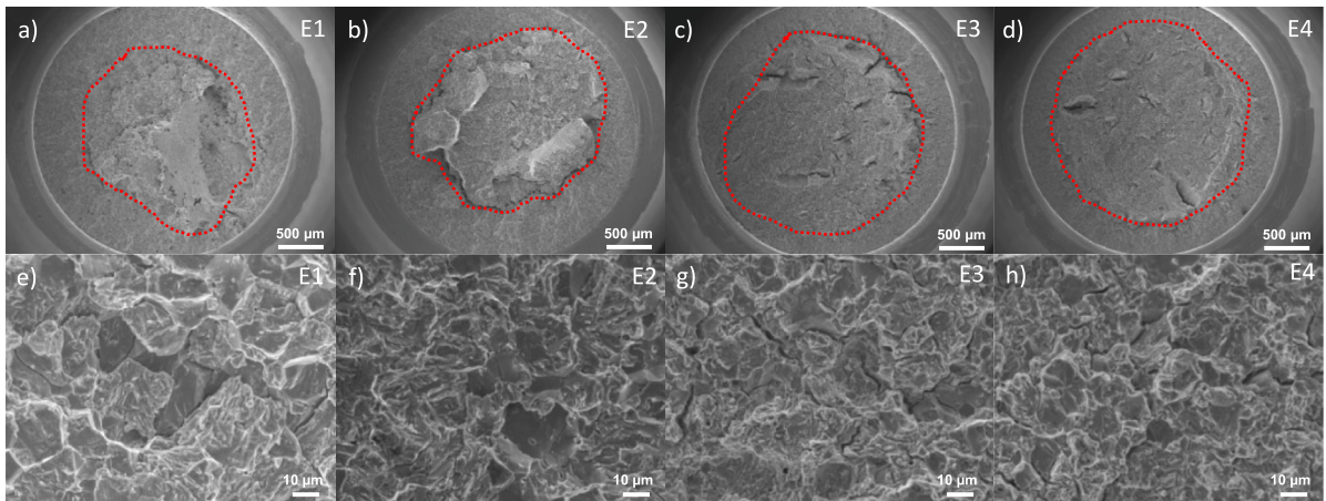
Fig. 4. (a, b, c, d) SEM photos of the whole fractured surfaces of specimens E1 to E4, respectively, during hydrogen charging (magnification 33\times ), and (e, f, g, h) the fractured surfaces at the edge of the specimens (magnification 1000\times ), in specimens E1 to E4, respectively).
