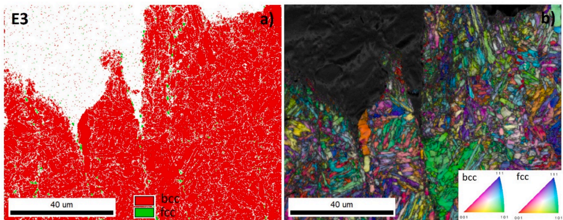
Fig. 8. EBSD phase maps of the axial plane of the E3 specimen containing the phases bcc (red) – martensite and delta ferrite, and fcc (green) – austenite (a), and the corresponding IPF + QI maps (b). The fracture is at the top. (For interpretation of the references to colour in this figure legend, the reader is referred to the web version of this article.)
