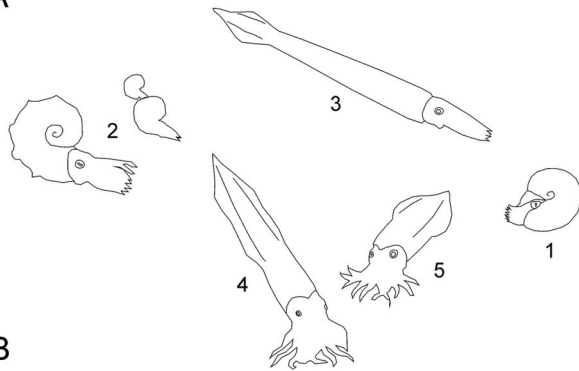
Fig. 10 A Reconstruction of cephalopod habitat within Western Carpathian Ráztoka Limestone, Illyrian Trinodosus—Reitzi Zones. Reconstruction: Petr Modlitba, with courtesy of author. B 1. Nautiloids. 2. Diverse ammonoids. 3. Aulacoceratids. 4. Mojsisovicsteuthis . 5. Breviconoteuthis . The benthic fauna is composed by abundant crinoids, echinoids, bivalves and brachiopods. Algae meadows are supposed based on geochemical data. C Fragment of partly tectonically deformed phragmocone of undetermined aulacoceratid; scale bar equals 1 cm
