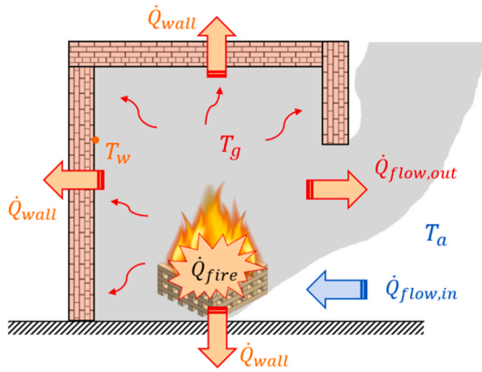
Fig. 3. Side view schematisation of heating phase.
