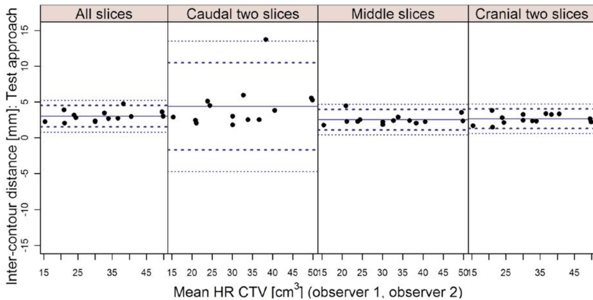
FIGURE 3. Bland-Altman inter-observer analysis of the distances between contours for conventional (A) and test (B) approach and for different levels of the contoured volume (all, caudal two, middle and cranial two slices). Full circles: mean values (mm) of the individual distances. Thick dotted lines: limits of agreement (mean \pm 2 standard deviations). Thin dotted lines: 95% confidence limits.
