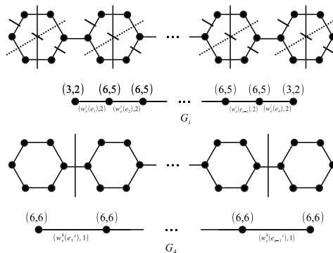
Figure 2. Strength-weighted quotient graphs G_i, i \in \{1, 2, 3\} , and G_4 of the graph PPC_n .
