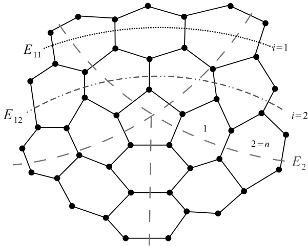
Figure 3. Carbon nanocone CNC_5(2) .
