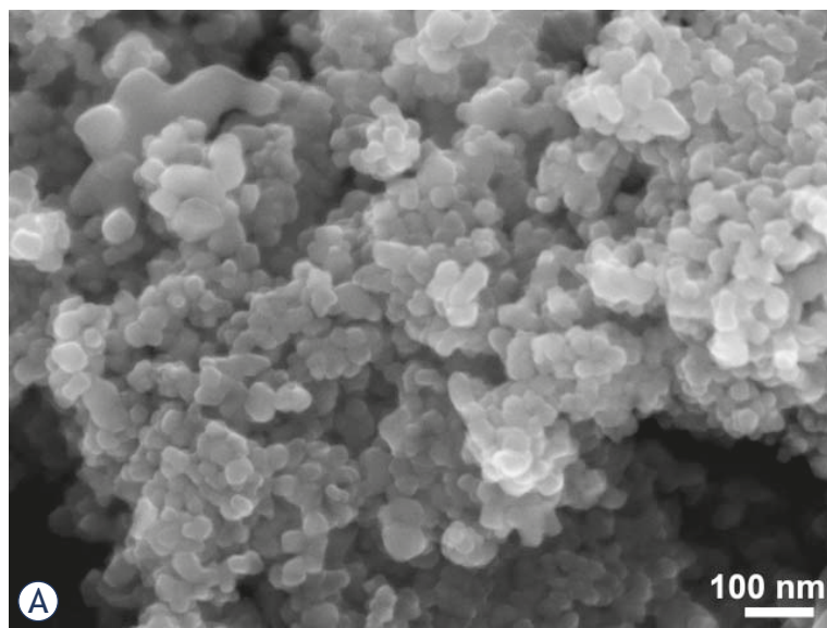
FIGURE 2. Field emission electron micrographs of the powders from two commercial sunscreens: A-SPF 20 (A) and N-SPF 10 (B), and their XRD diffraction (C).
