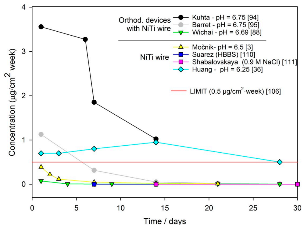
Figure 6. Concentration of Ni ions vs. time of immersion for data reported at pH ~7.
