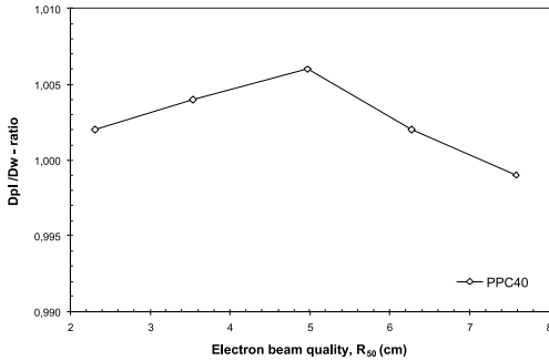
Figure 1. Ratios D_{pl}/D_w of absorbed doses determined with measurements in Plastic Water and in water for five high-energy electron beams - electron beam qualities. Measurements were performed with plane parallel ionisation chamber PPC40. Beam data are in Table 2.
