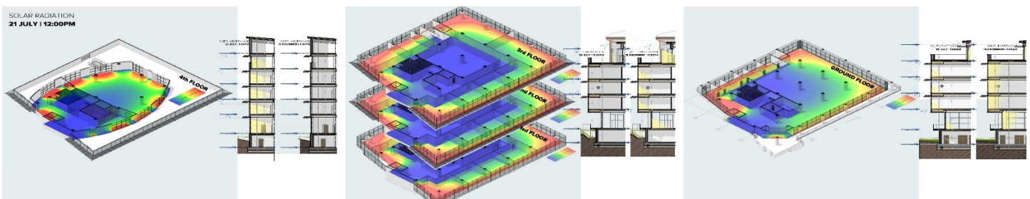
Figure 4. Analysis of solar radiation
