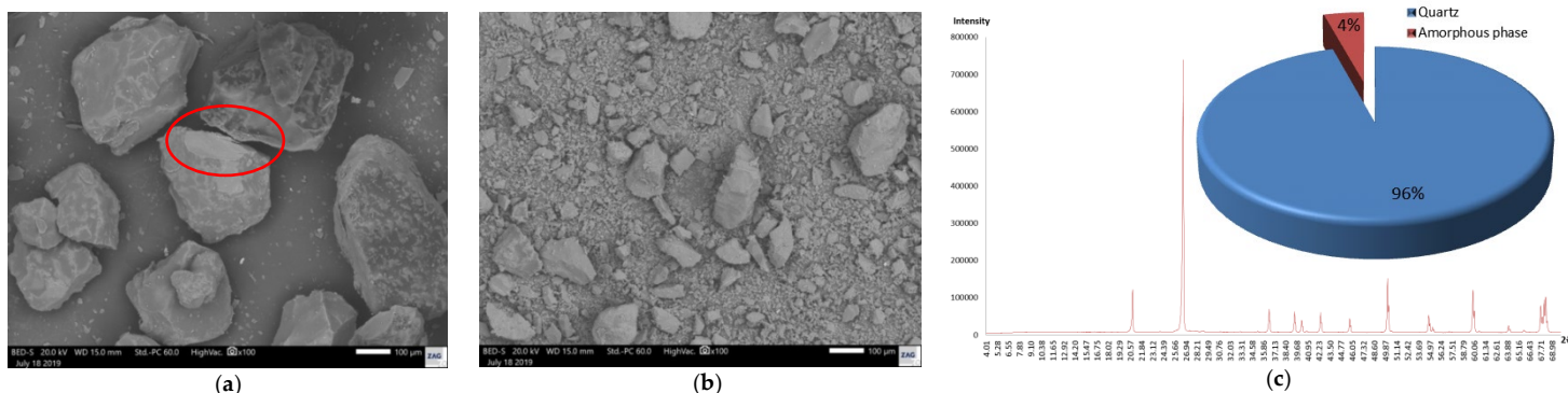
Figure 1: SEM micrographs of WCC. (a) Gently ground in a mortar with pestle and sieved below 600 μm (red circle: damaged surface); (b) ground in vibrating disk mill and sieved below 90 μm, (c) XRD pattern of WCC and on the inset its Rietveld refinement.
