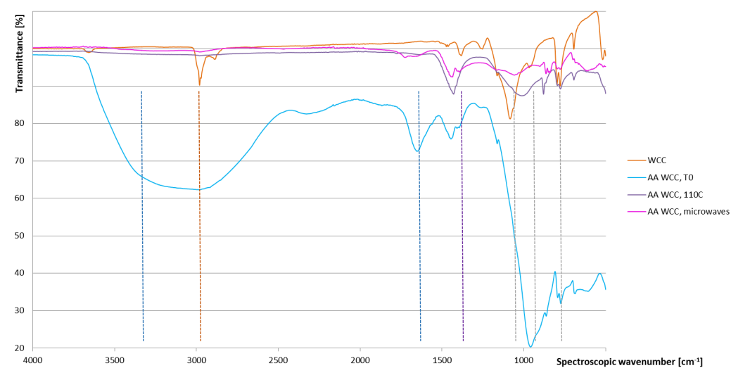
Figure 7: FTIR of precursor and AAM dried with different methods. Blue lines O-H bonds, orange lines C-H bonds, dashed purple lines aromatic C-H 2 and C-H 3 bond, grey lines Si-O bonds.
