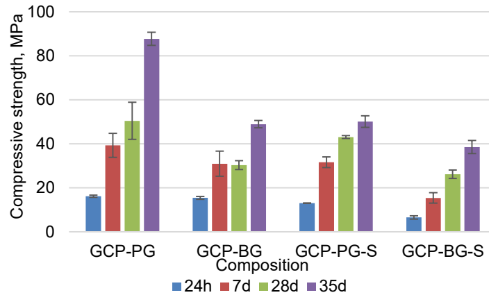
Figure 2. The compressive strength of ternary binder and mortar.
