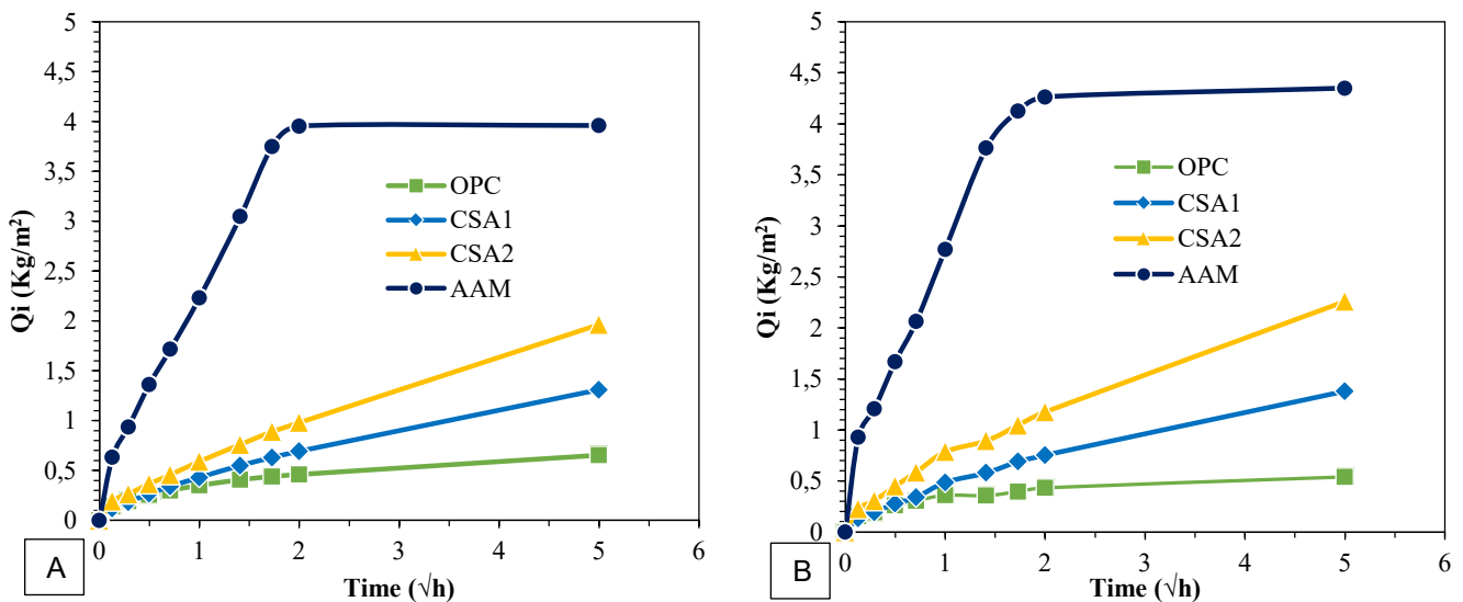
Figure 2: Water absorbed per unit area at (A) 28 days (B) 56 days.
