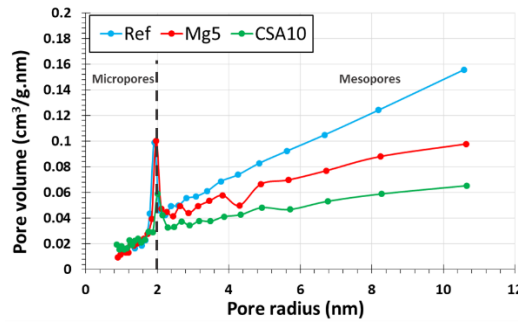
Figure 4: Pore distribution measured by sorption analysis.
