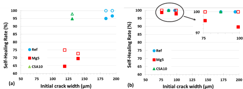
Figure 5: Self-Healing Rate for Ref , Mg5 and CSA10 after 35 days (●) and 120 days (○) of healing for the bottom (a) and lateral (b) cracks.
