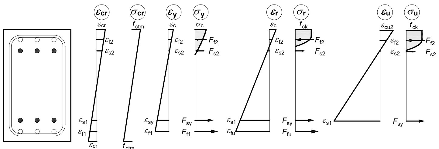
Figure 2: Strains and internal forces for specific points of bending moment – curvature diagram
