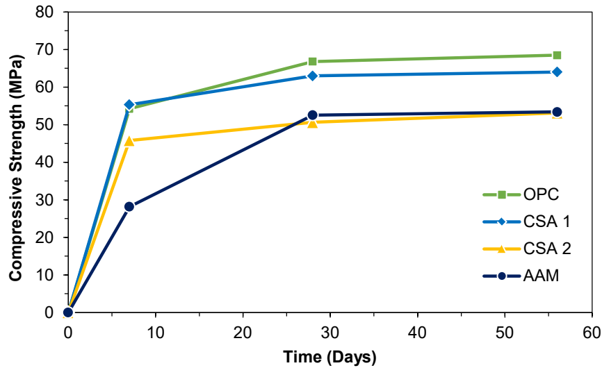
Figure 1: Strength development of different binder systems over time
