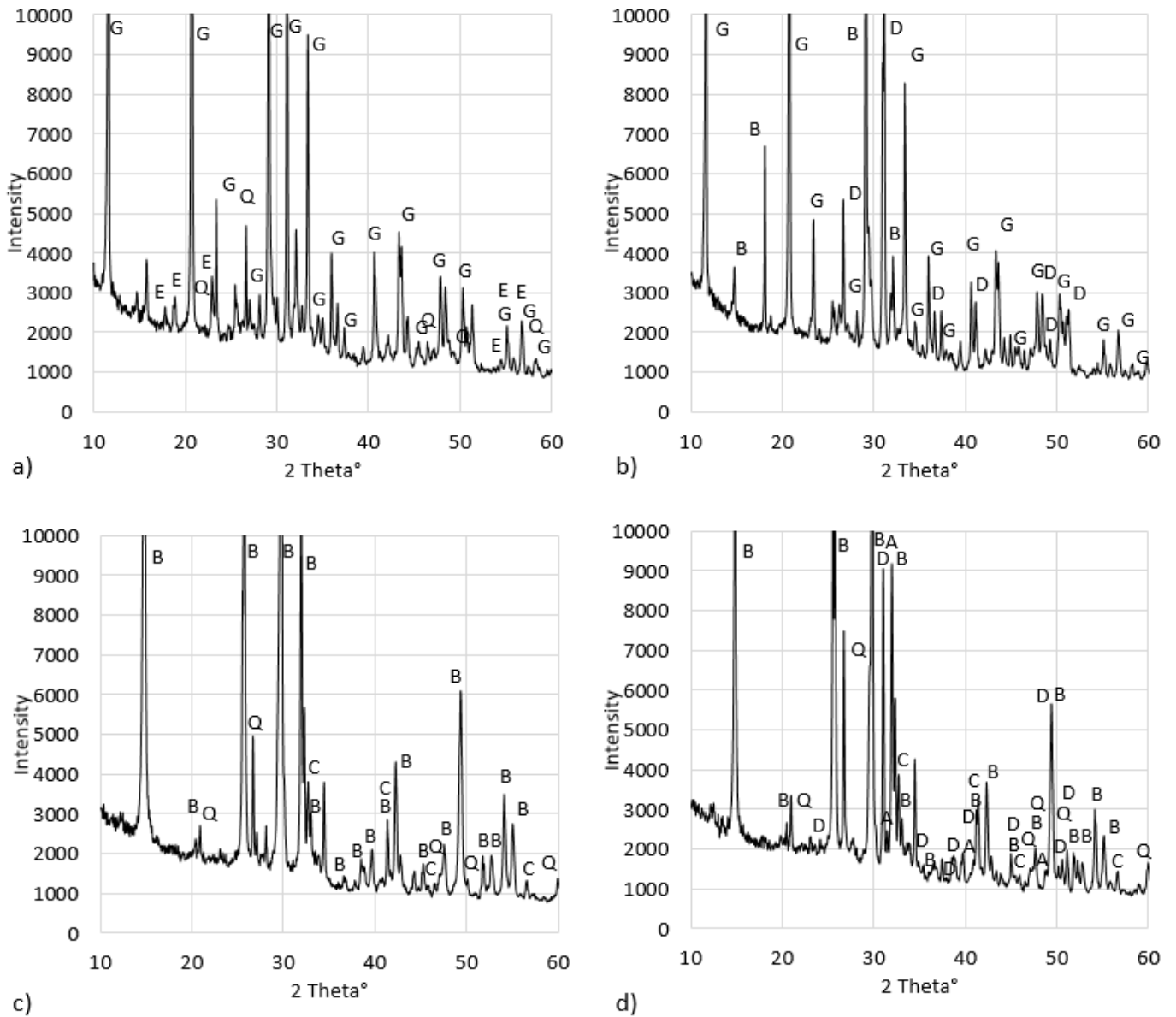
Figure 5. Mineralogical characterisation of raw material mixture and hydrated paste of ternary binder: a) Hydrated GCP-PG; b) hydrated GCP-BG, c) raw mixture of GCP-PG, d) raw mixture of GCP-BG. B- Bassanite ( \text{CaSO}_4 \cdot 0.5\text{H}_2\text{O} , ref 33-0310), C - calcium silicate oxide ( \text{Ca}_3(\text{SiO}_4)\text{O} , ref 73-0599), Q - quartz ( \text{SiO}_2 , ref 78-1252), D - dolomite ( \text{CaMg}(\text{CO}_3)_2 , ref 36-0426), A - anhydrite ( \text{Ca}(\text{SO}_4) , ref 72-0916), G - gypsum ( \text{Ca}(\text{SO}_4)(\text{H}_2\text{O})_2 (74-1433), E - ettringite ( \text{Ca}_6(\text{Al}(\text{OH})_6)_2(\text{SO}_4)_3(\text{H}_2\text{O})_{26} , ref 72-0646).
