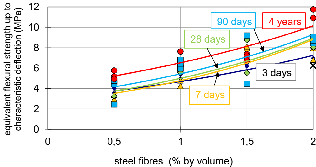
Figure 5: Correlation of the quantity of steel fibres and equivalent strength to the characteristic deflection \bar{\sigma}_{\Delta\delta} at different ages of SFRC
