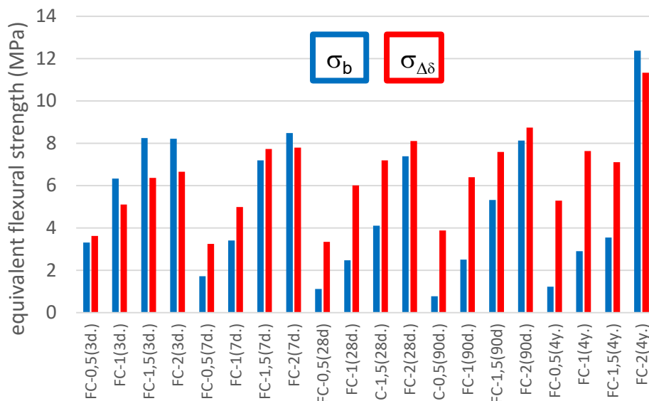
Figure 6: Comparison of average equivalent flexural strengths \bar{\sigma}_b and \bar{\sigma}_{\Delta\delta} at individual ages of SFRC
