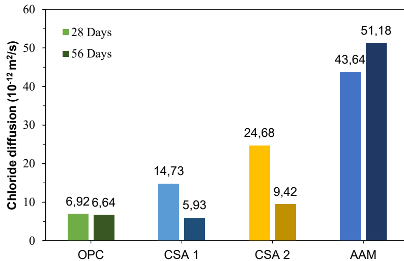
Figure 4: Chloride diffusion of different binder systems at 28 days 56 days.
