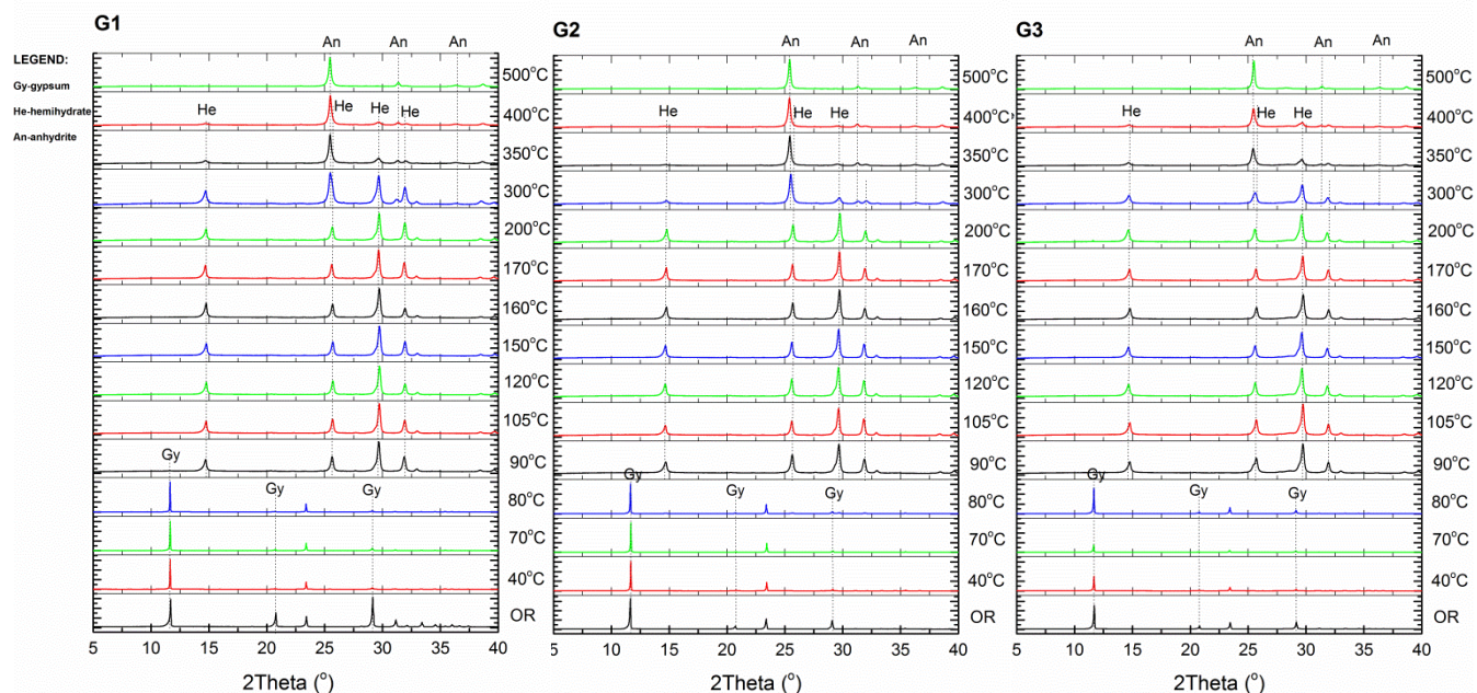
Figure 2: XRD patterns of the synthetic gypsum powders, pre-treated at different temperatures (OR: non-treated powder)
