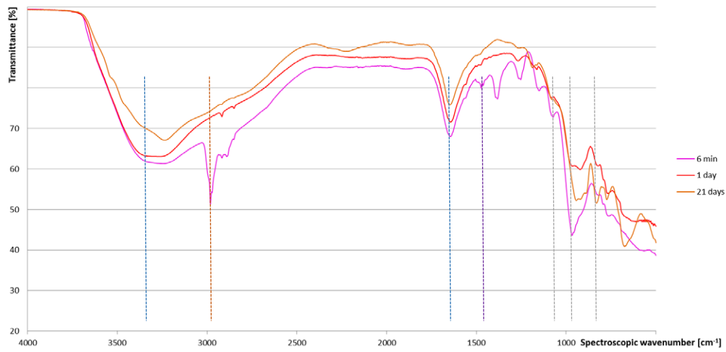
Figure 8: FTIR time dependence of AAM dried at room temperature. Blue lines O-H bonds, orange lines C-H bonds, dashed purple lines aromatic C-H 2 and C-H 3 bonds, grey lines Si-O bonds.
