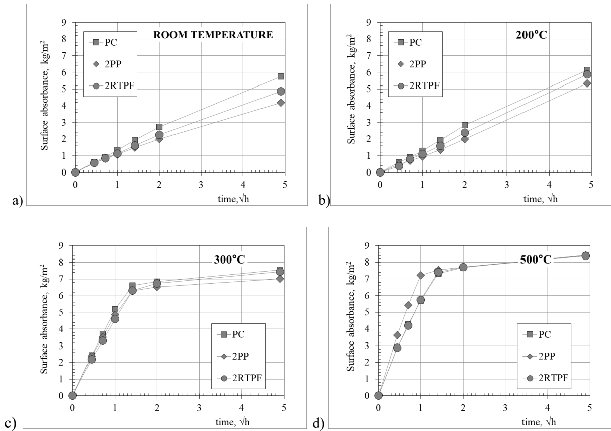
Figure 4 Changes in capillary absorption of PC, 2PP and 2RTPF concrete at a) room temperature and after exposure to temperatures b) 200°C, c) 300°C and d) 500°C
