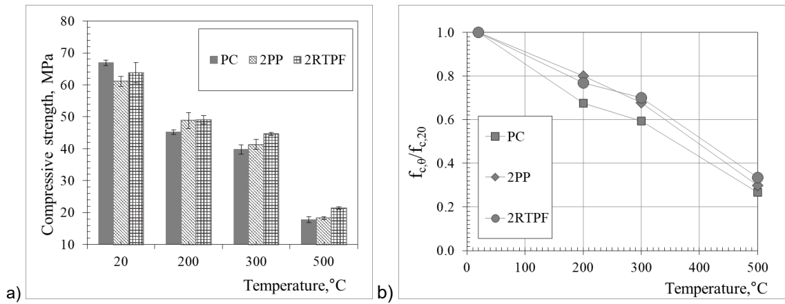
Figure 1 Residual compressive strength vs temperature a) mean and b) relative values
