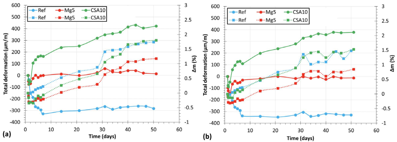
Figure 3: Total deformation (continuous line) and mass variation (dotted line) of the three studied mortars stored under WC (a) and CC (b)
