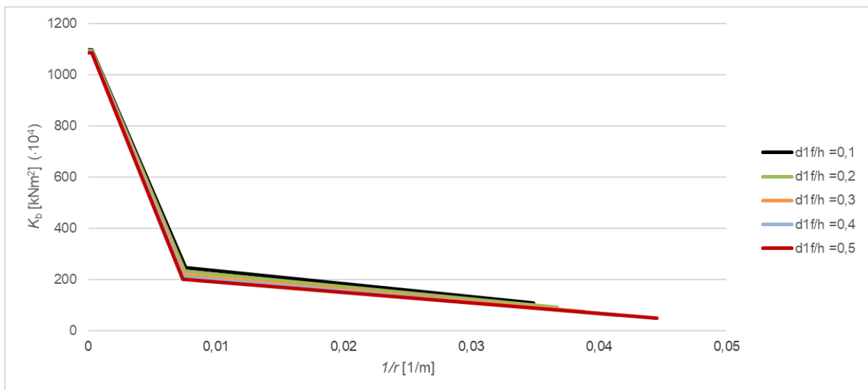
Figure 6. Bending stiffness – curvature diagram with the change of GFRP location
