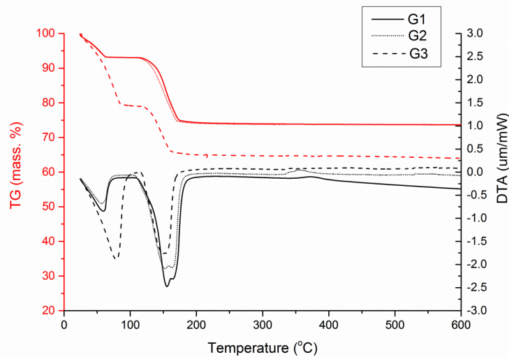
Figure 1: Thermal curves of the synthetic gypsum powders
