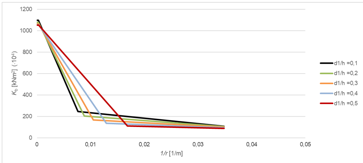
Figure 5. Bending stiffness – curvature diagram with the change of steel location
