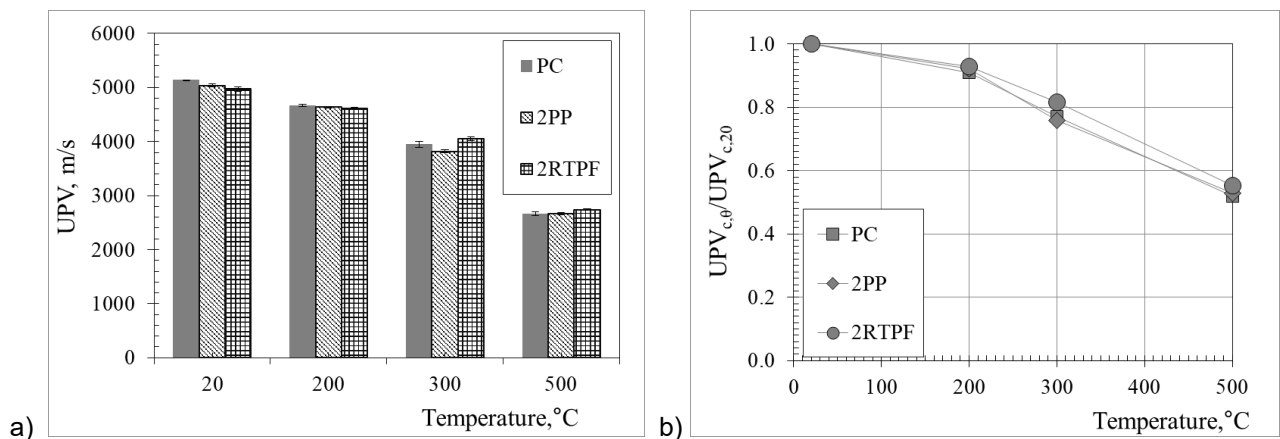
Figure 3 Residual UPV of tested concrete a) mean and b) relative values
