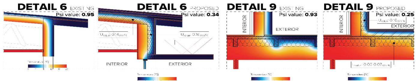
Figure 7. Thermal bridges (detail 6 is for intervention M2 and detail 09 is for M1)
