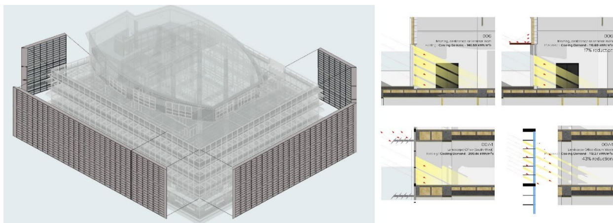
Figure 9. New structure of the facade and Integration of shading devices in 4th floor after the intervention (M.4 and M.8)
