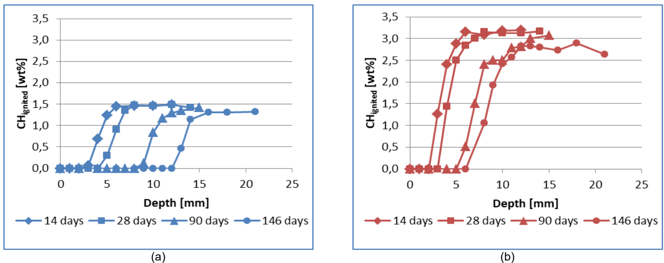
Figure 3: CH content measured with thermogravimetric analysis (TGA) after 14, 28, 90 and 146 days of exposure to accelerated carbonation for (a) EnDurCrete mortar (EnM-06) and (b) reference mortar (RefM-06) both made with w/c ratio of 0.6.
