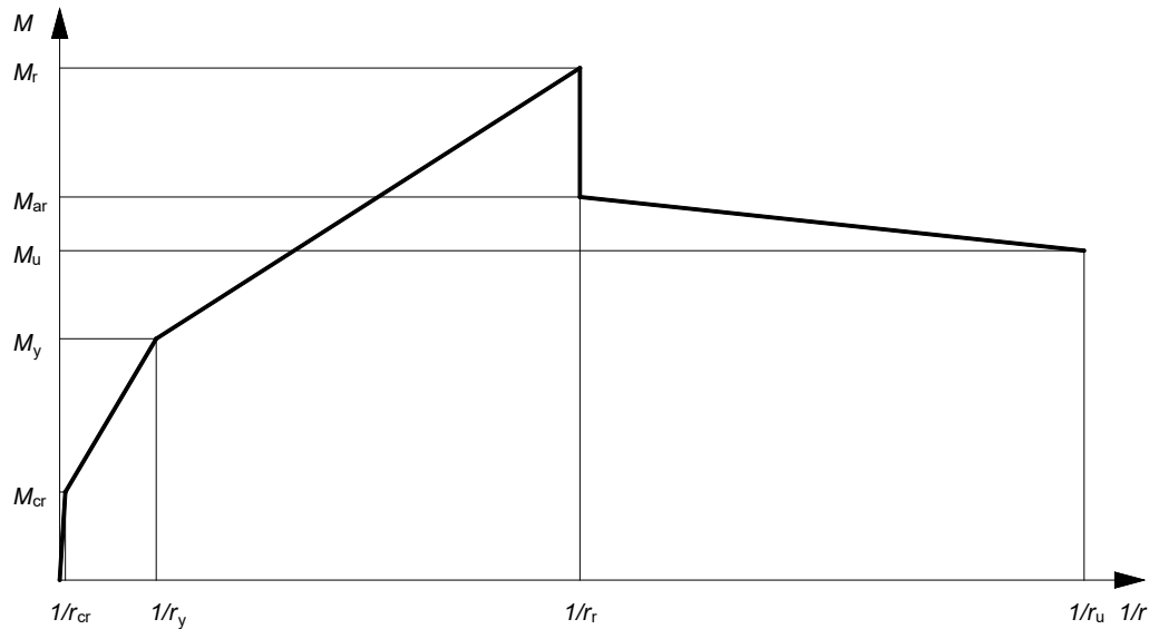
Figure 3. Bending moment – curvature diagram for failure mode 6
