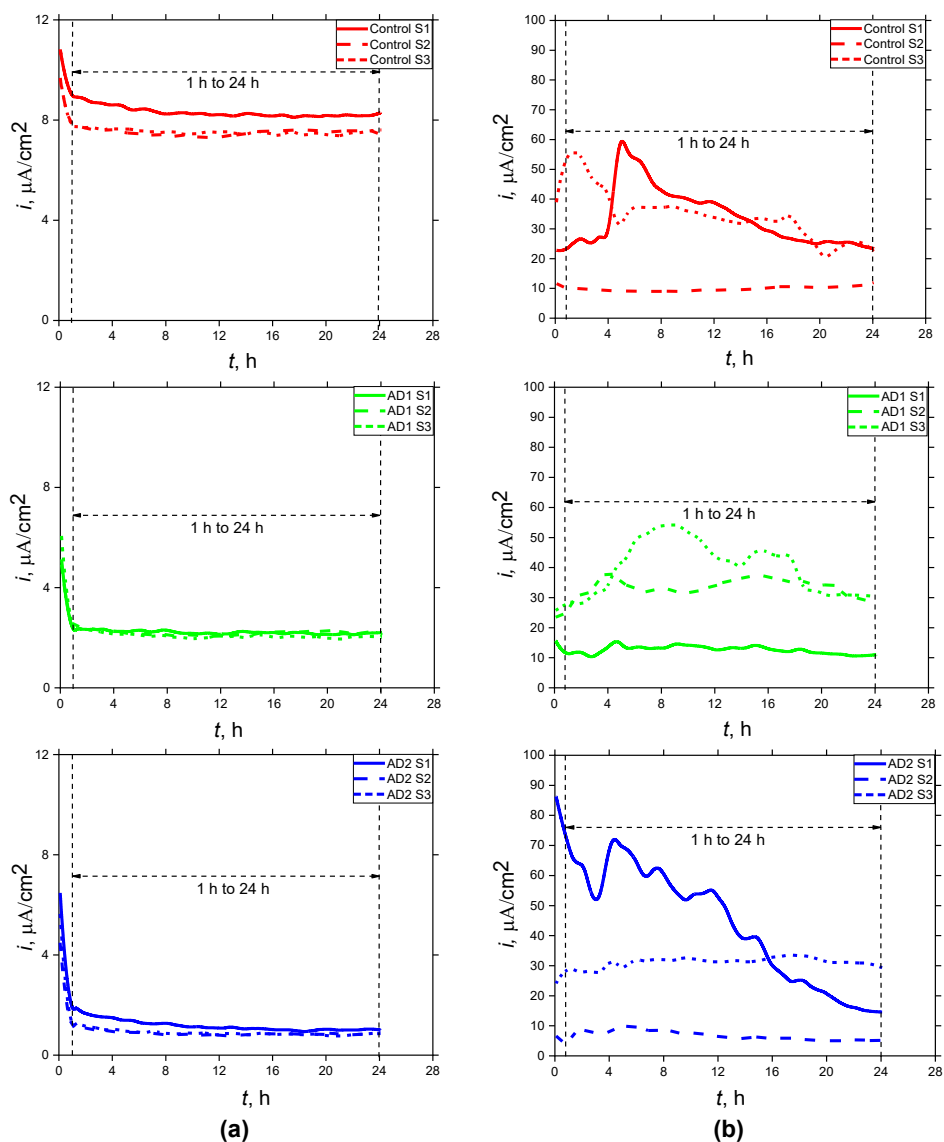
Figure 3 Current density values from EN 480-14 method and specimen exposed to a) Sat. Ca (OH) 2 b) 3.5% NaCl solution
