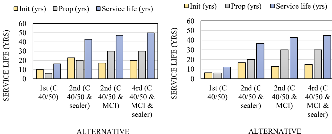
Figure 1 Prediction of the service life for concrete columns exposed to: a) marine spray zone, b) marine tidal zone.
