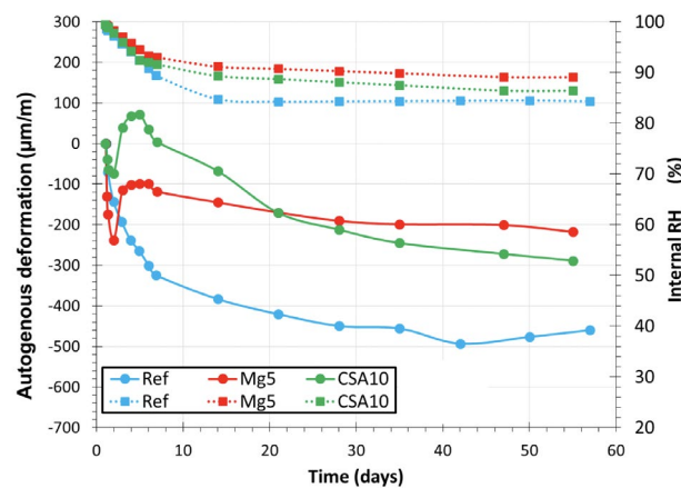
Figure 2: Evolution of the autogenous deformation (continuous line) and the Internal Relative Humidity (IRH - dotted line)
