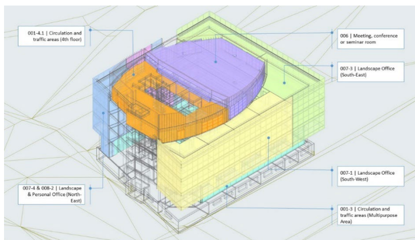
Figure 6. Thermal zones with high demand for cooling
