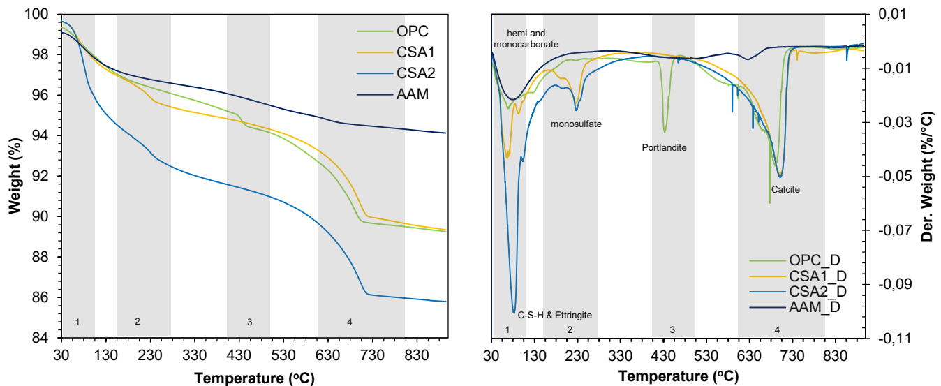
Figure 5: (A) TG thermograms and (B) DT thermograms for all systems.
