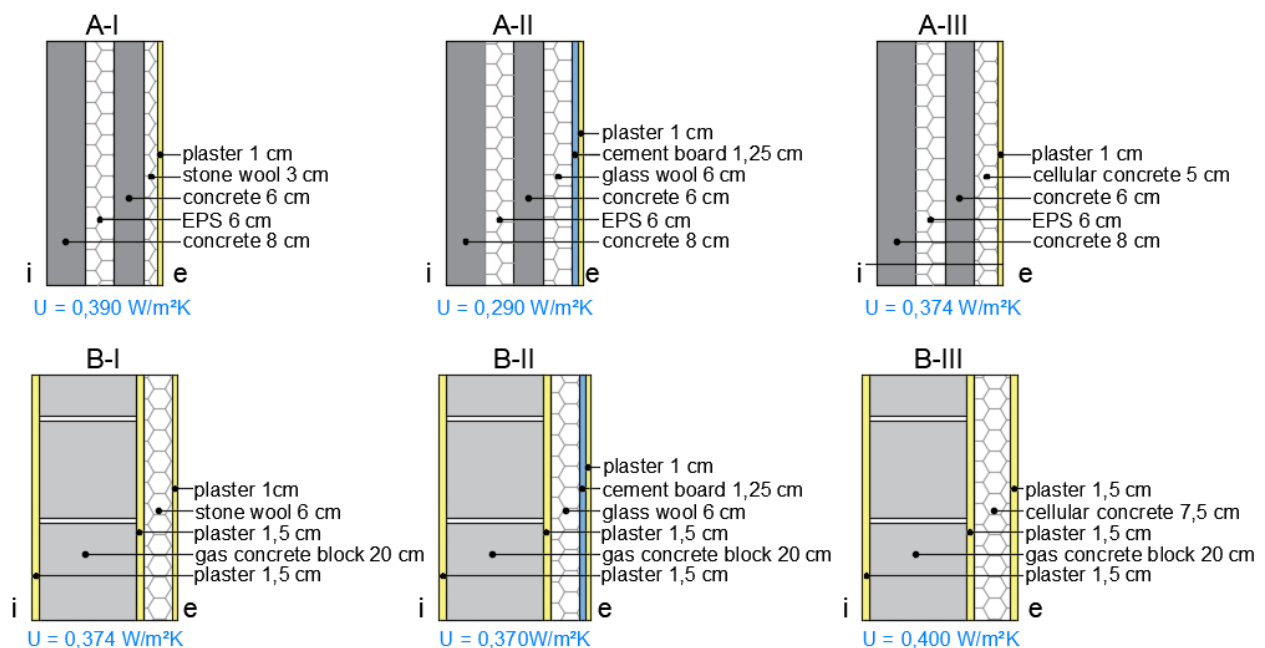
Figure 2: Proposed façade systems with improved U-values
