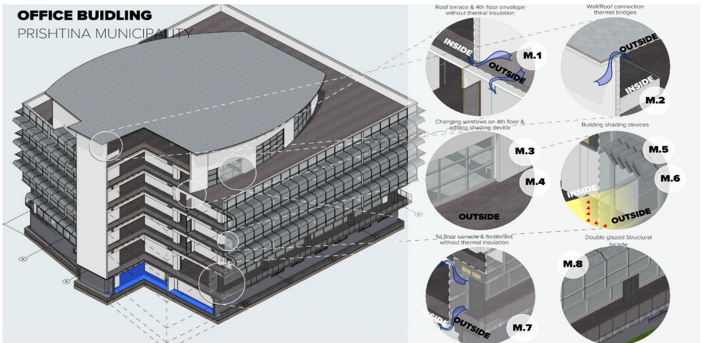
Figure 3. Possible intervention to reduce the energy demand
