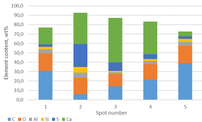
Figure 6. EDX analysis of GCP-PG binder
