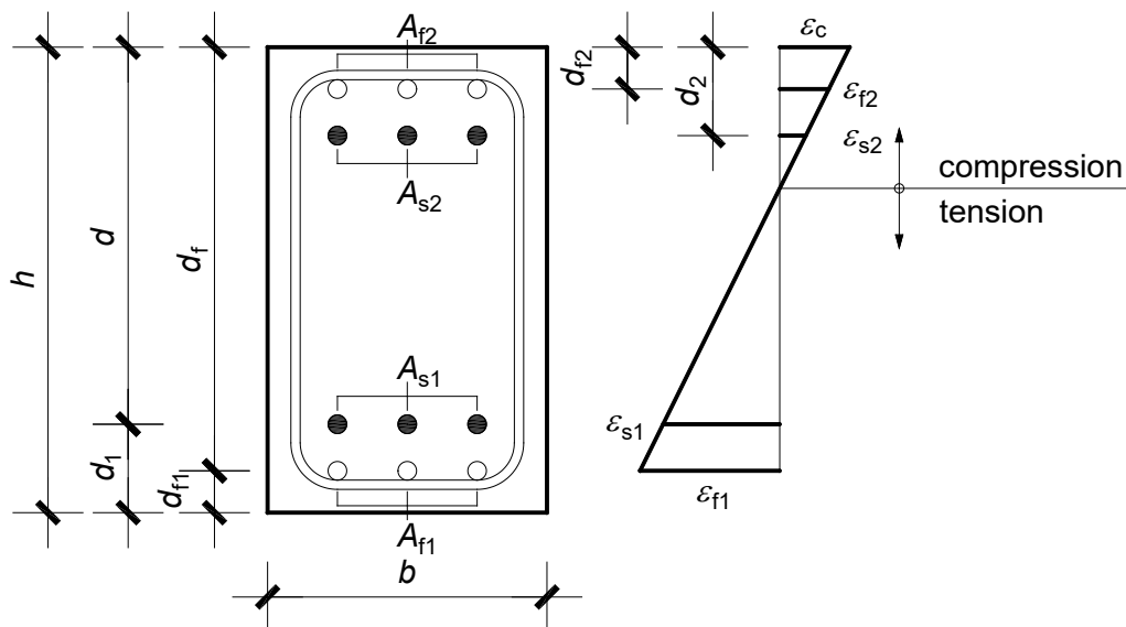
Figure 1: Section geometry and strains
