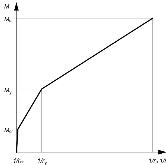
Figure 4. Bending moment – curvature diagram for failure mode 2 occurring in analysis
