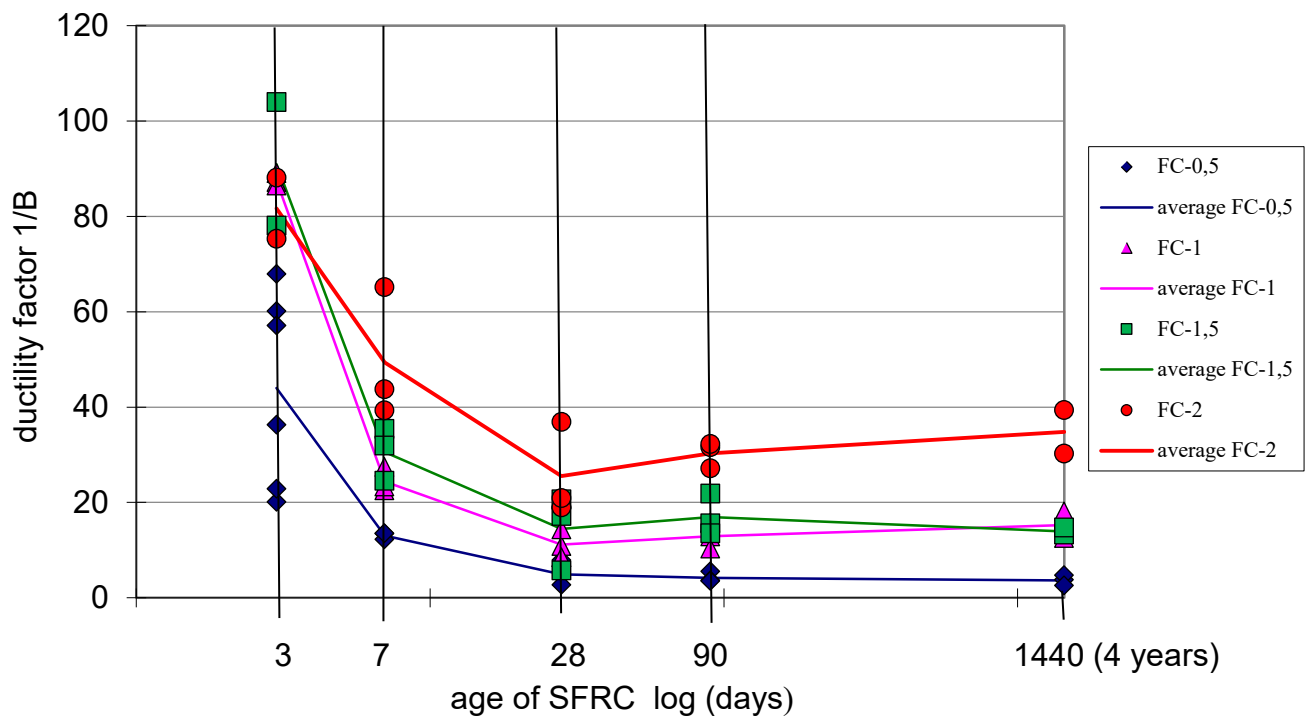
Figure 4: Correlation of ductility factor 1/B, SFRC age and steel fibre volume percentage
