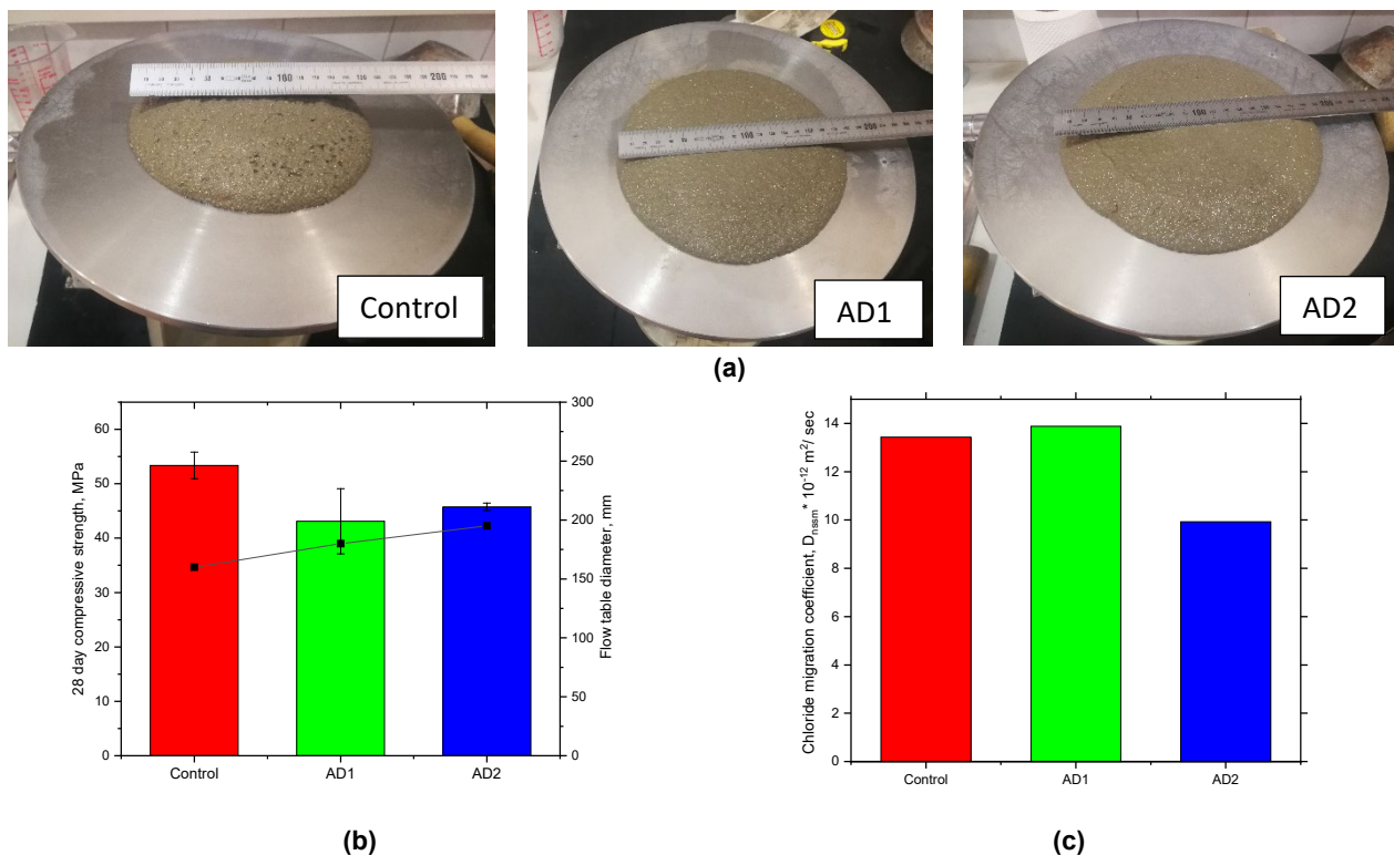
Figure 2 a) Flow table result of each mix, b) 28-day compressive strength and flow table diameter of each mix c) 28-day chloride migration coefficient of each mix
