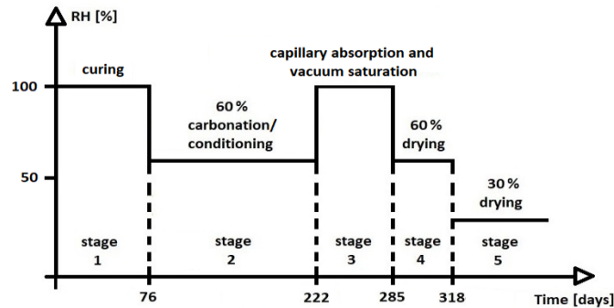
Figure 1: Stages of the moisture transport experiment carried out on the thin plates.
