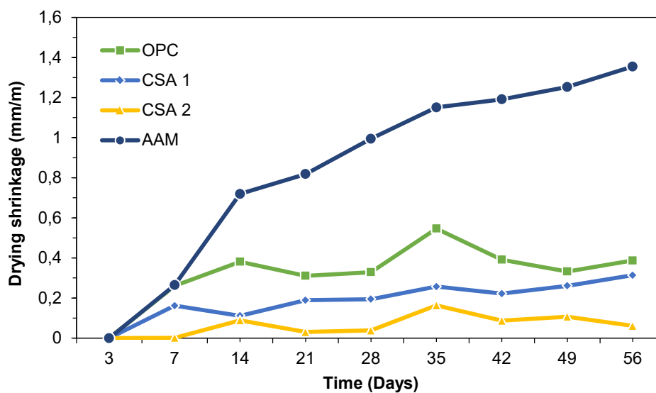
Figure 3: Drying shrinkage of different binder systems at different ages
