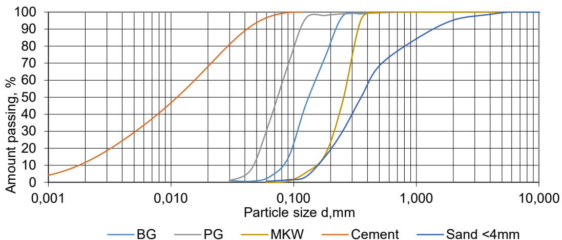
Figure 1. The article size distribution of the raw materials used to prepare novel building material.
