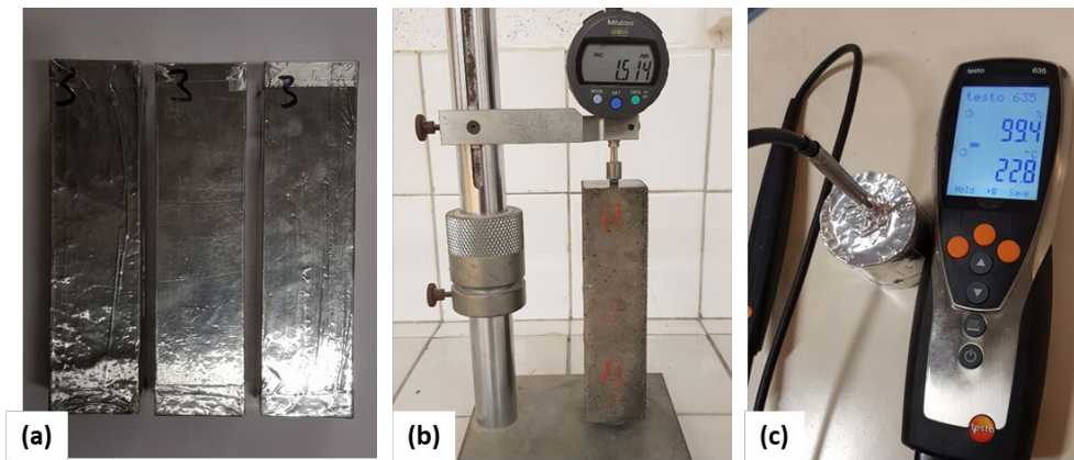
Figure 1: Specimens with a double layer of aluminum foils (a) – Retractor for length measurement (b) – Internal Relative Humidity (IRH) measurement (c).
