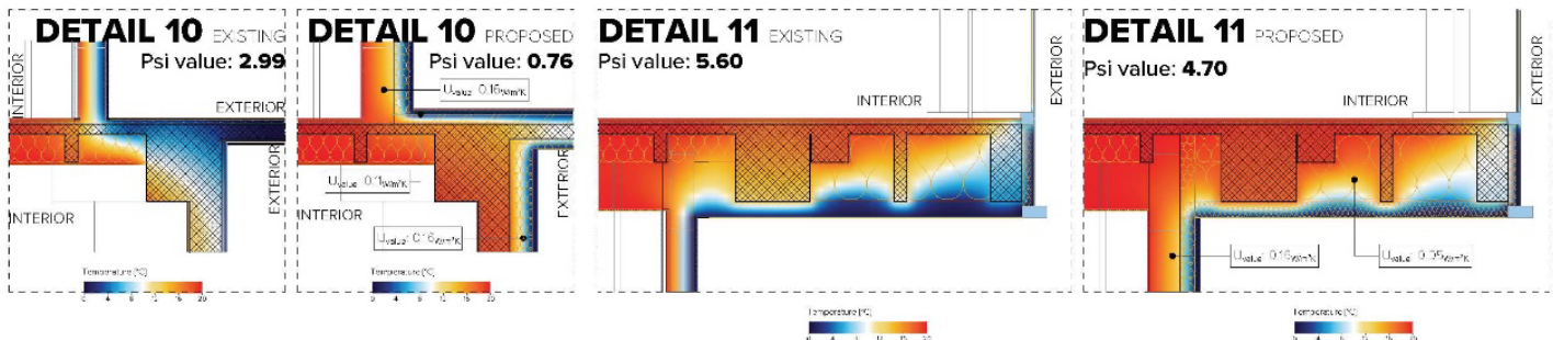
Figure 8. Thermal bridges between walls, floor and ceiling of M.7 intervention
