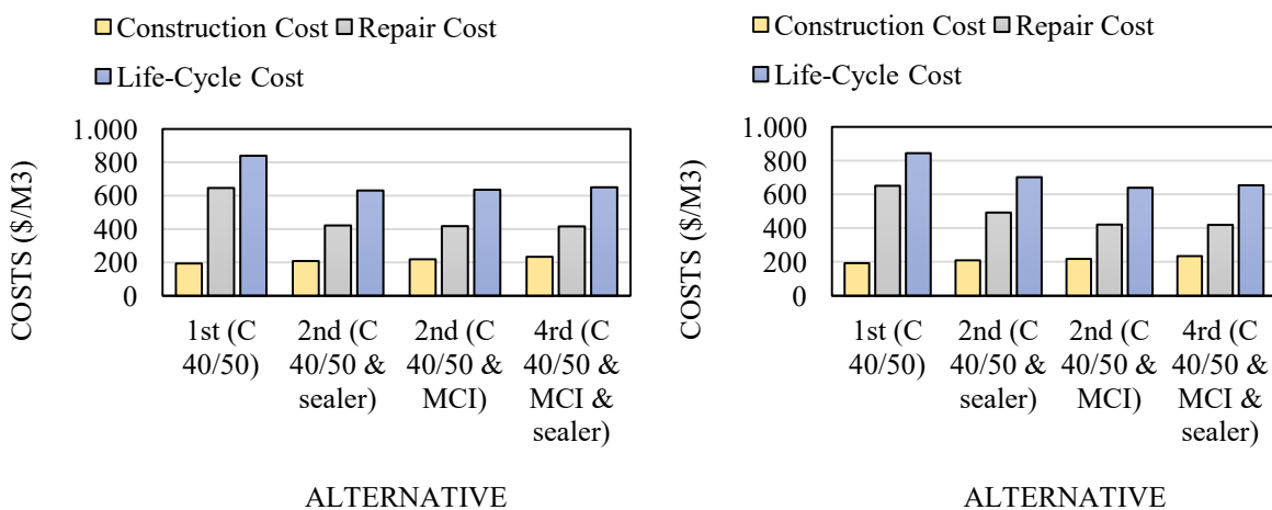
Figure 2 Life cycle costs for concrete columns exposed to: a) marine spray zone, b) marine tidal zone.
