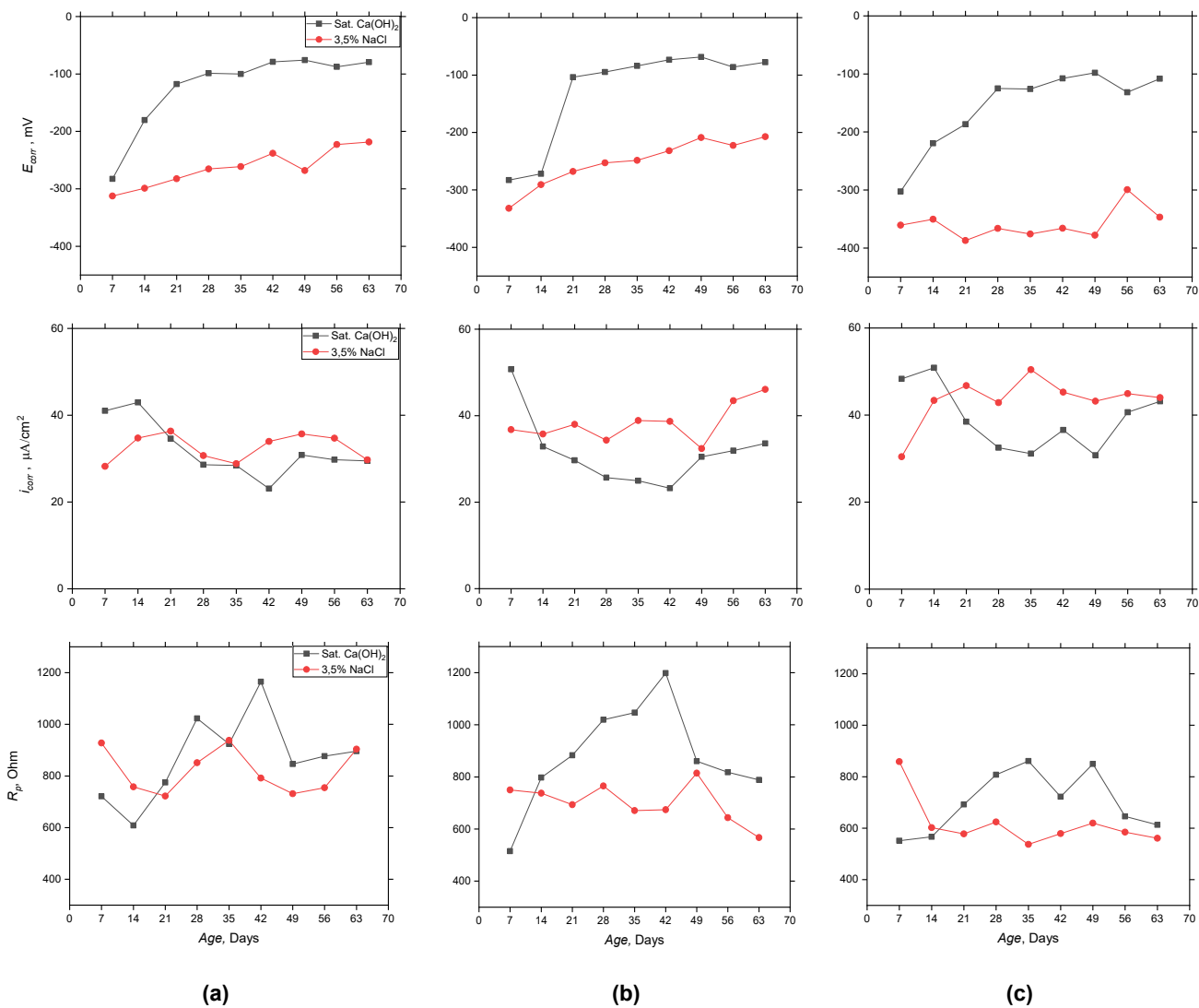
Figure 4 Open circuit potential ( E_{ocv} ), current density i_{corr} and polarization resistance R_p obtained using alternative method for a) Control specimen b) AD1 specimen and c) AD2 specimen
