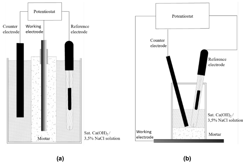
Figure 1 Schematic test set up two testing approaches a) Standardized method, b) Alternative method
