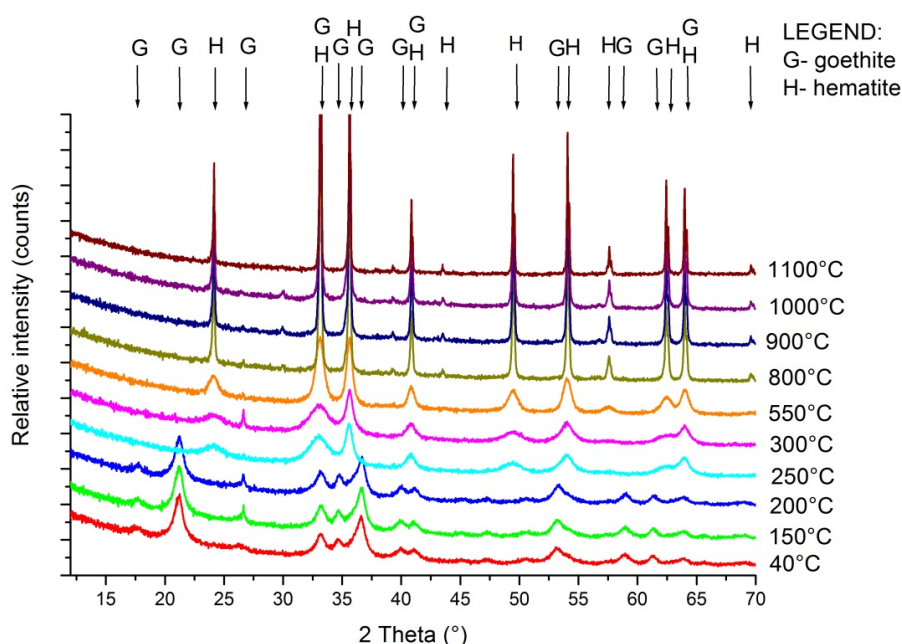
Figure 1: XRD patterns of an investigated sample of pigment annealed at different temperatures
