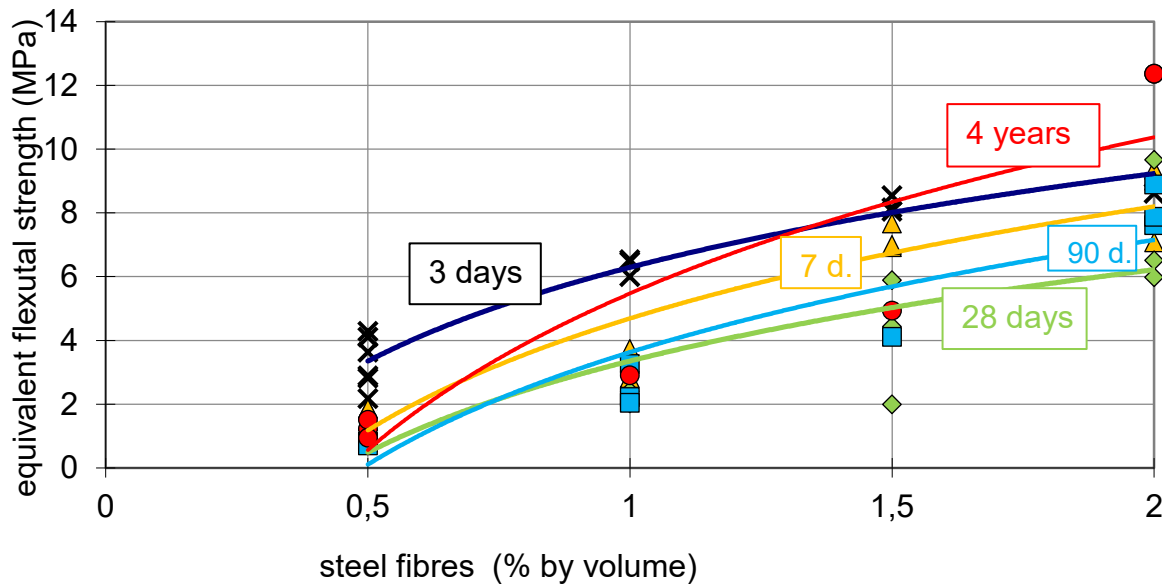
Figure 3: Ratio of equivalent flexural strength \bar{\sigma}_b of SFRC of different ages and volume percentage of added steel fibres
