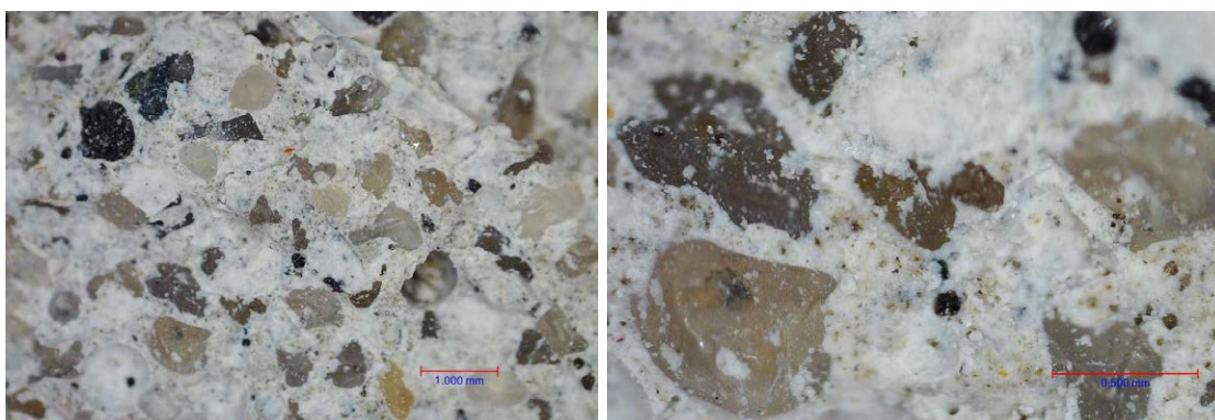
Figure 3. Typical macrostructure of the ternary system mortar.
