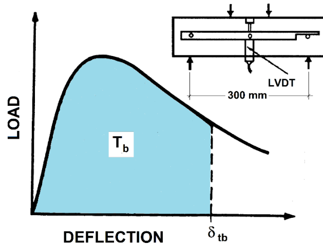
Figure1: Schematic diagram of the load-deflection and test configuration according to the JCSE-SF4
