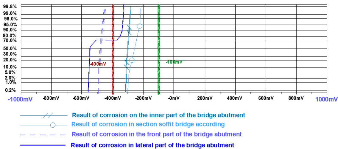
Figure 8. Results of the corrosion rate in specific positions.
