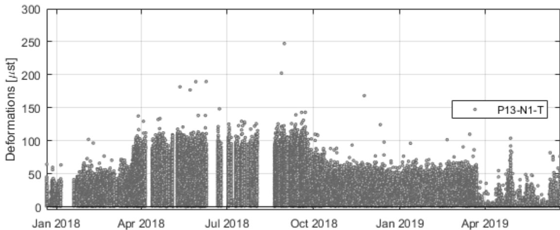
Figure 6: Traffic induced strains for beam in field number 13 of the right viaduct
