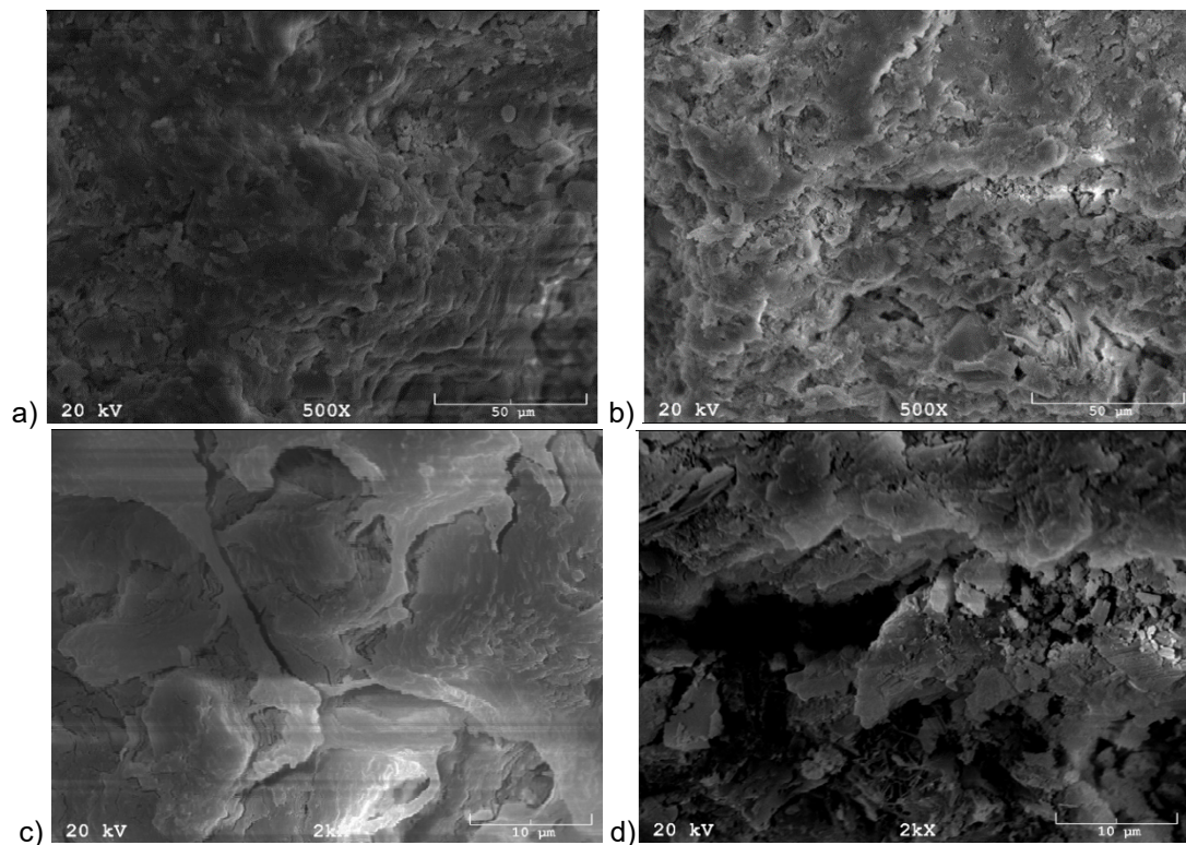
Figure 4: Microstructure of the ternary binder detected by SEM in magnification of 500x and 2000x. a), c) GCP-PG, b), d) GCP-BG.
