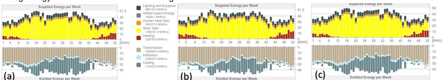
Figure 5. (a) Project of energy balance for current situation for the office building of Prishtina Municipality, (b) Peja, (c) Ferizaj
