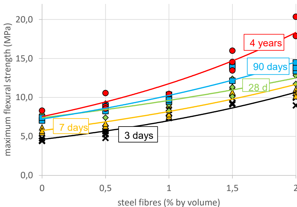
Figure 2: Increasing the value of f_{max} , concrete of different ages, depending on the volume percentage of steel fibres
