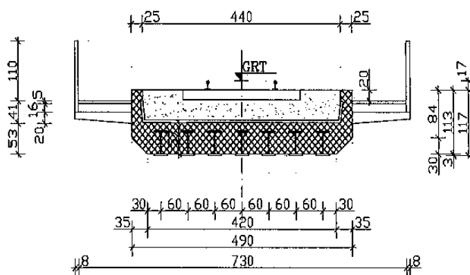
Figure 5: New Buna bridge
