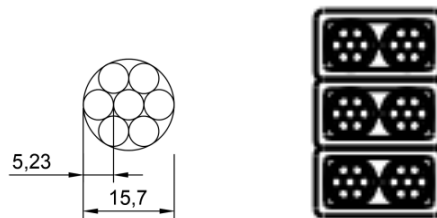
Figure 7: 7-wire prestressing steel strand (left) and prestressing cable with 3 HDPE tubes and overall 6 strands
