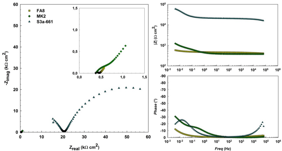
Figure 5: Representative EIS spectra recorded in 17 th wetting / drying cycle in three alkali-activated mortars.
