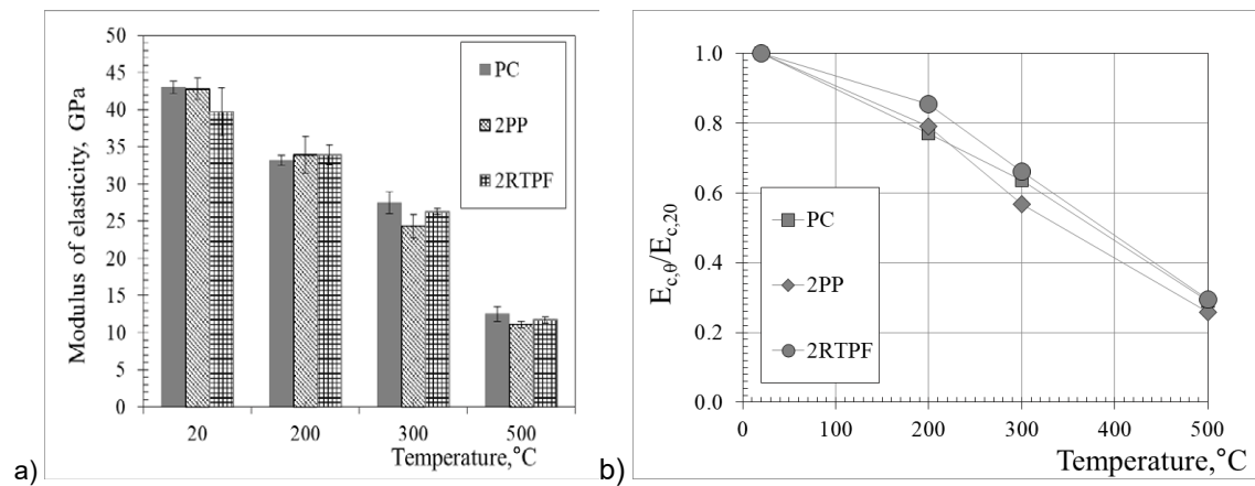
Figure 2 Residual modulus of elasticity vs temperature a) mean and b) relative values
