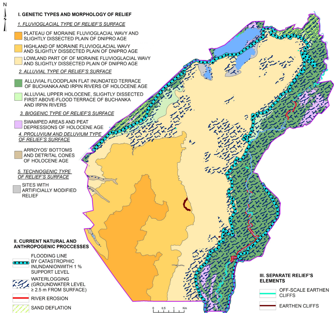
Fig. 2. Geomorphological map of Irpin city (Zhyrnov & Solomakha, 2022).
