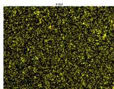
(b-K)
