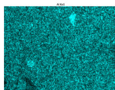
(b-Al)
