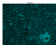
(b-Mg)
