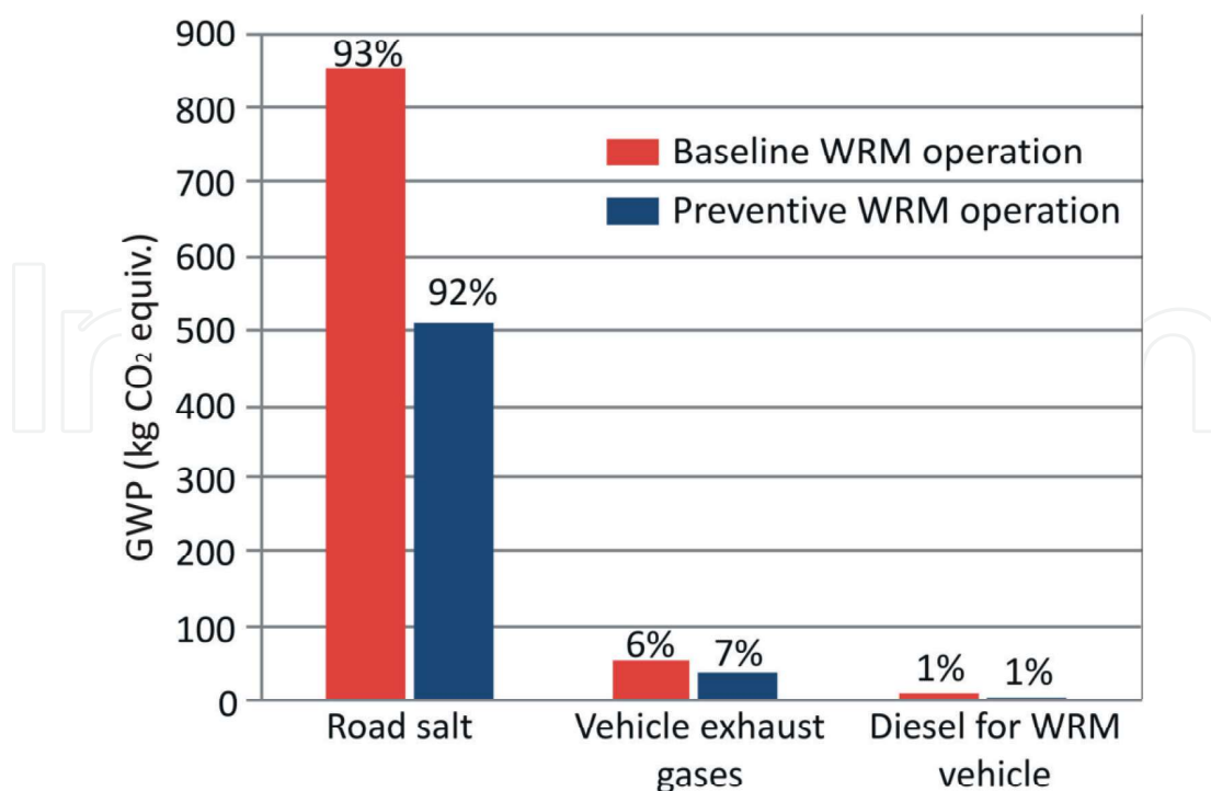
Figure 3. Global warming potential associated with the operation of WRM vehicle (salt gritting, fuel consumption, and related exhaust gases) in two benchmarked scenarios.
