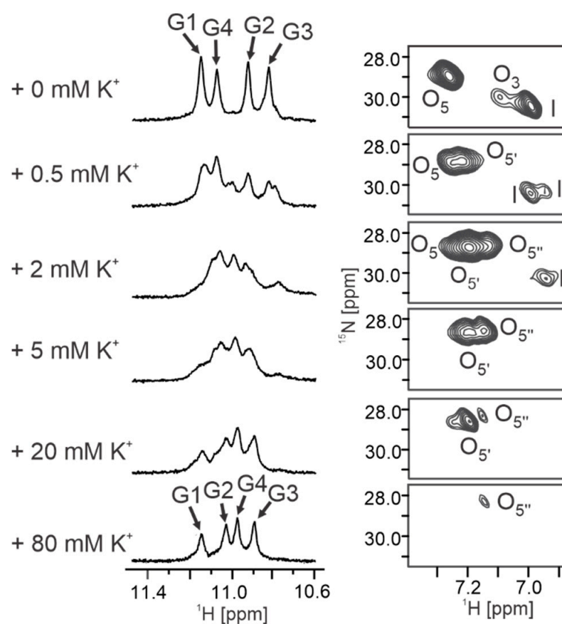
Figure 6. Imino regions of ^1\text{H} NMR and corresponding ^1\text{H} - ^{15}\text{N} HSQC spectra of [\text{d}(\text{G}_4\text{C}_2)]_4 at 25 °C, pH 6.0, in 10% ^2\text{H}_2\text{O} in the presence of 100 mM of ^{15}\text{NH}_4\text{Cl} and gradual addition of KCl. The oligonucleotide concentration was 2.0 mM per strand. Assignments of imino resonances at the beginning and end of titration are indicated above the signals. Annotations of cross-peaks are shown next to the peaks.
