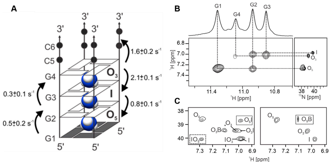
Figure 2. (A) Folding topology and cation binding sites within G-quadruplex adopted by d(G_4C_2) in the presence of ^{15}\text{NH}_4^+ ions, with the three ion binding sites shown. Syn - and anti -conformations of guanines are represented with grey and white rectangles, respectively. The arrows represent the observed movements between cation binding sites, with apparent rate constants depicted next to them. (B) Imino-aromatic region of the NOESY spectrum (left), showing cross-peaks between bound ^{15}\text{NH}_4^+ ions and nearby imino protons, and the 2D ^1\text{H} - ^{15}\text{N} HSQC spectrum (right) exhibiting cross-peaks corresponding to ^{15}\text{NH}_4^+ ions in different chemical environments within [d(G_4C_2)]_4 . The vertical and horizontal dashed lines connect resonances of guanine imino and ^{15}\text{NH}_4^+ ion protons. (C) The 2D ^1\text{H} - ^{15}\text{N} NzExHSQC spectrum at a mixing time ( \tau_m ) of 1.1 s (left) and the 2D ^1\text{H} - ^{15}\text{N} HzExHSQC spectrum at a mixing time ( \tau_m ) of 40 ms (right). Annotations of autocorrelation and exchange cross-peaks are shown next to the cross-peaks.
