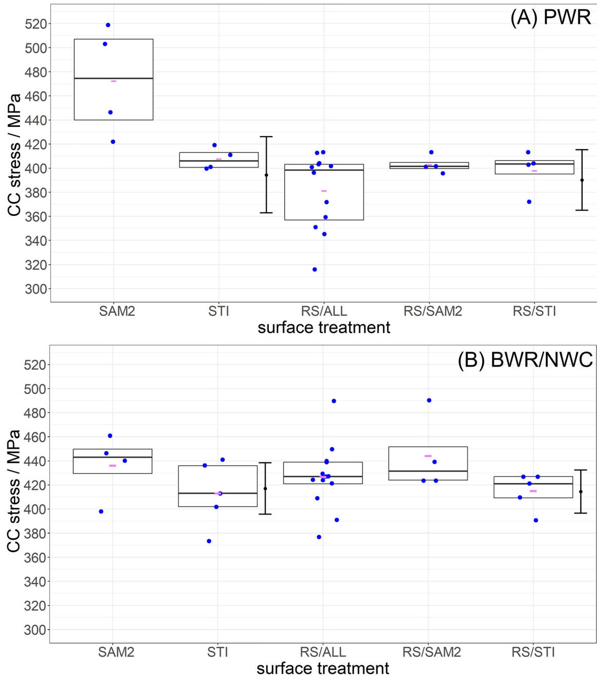
Figure 9: Summary of the measured EAC critical stress and calculated CC stress data dependence on surface treatments for Alloy 182 in (A) PWR and (B) BWR/NWC environments. The average value within each category is marked by a red dash, two error bars indicate CC stress obtained by extrapolation to zero strain rate. Other details are described in Section 3.3.
