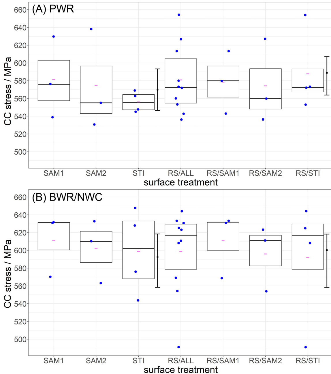
Figure 8: Summary of the measured EAC critical and calculated CC stress data dependence on surface treatments for CW 316L SS in (A) PWR and (B) BWR/NWC environments. The average EAC critical stress value within each category is marked by a red dash, two error bars indicate CC stress obtained by extrapolation to zero strain rate. Other details are described in Section 3.3.
