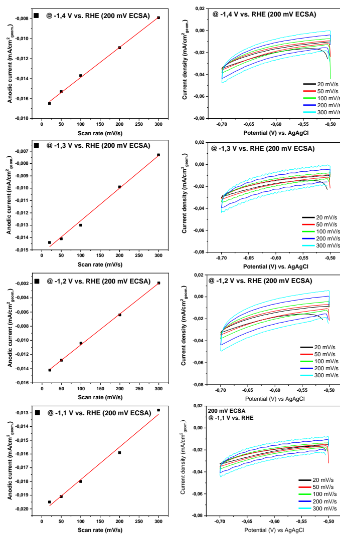
Figure S11. Linear plots of anodic current versus scan rates at the various potentials for Cu NCs-OCP200 sample with the corresponding cyclovoltammograms of 200 mV potential window (-0.7 to -0.5 V vs. Ag/AgCl). The anodic currents were taken at the middle window potential of -0.6 V vs. AgAgCl.
