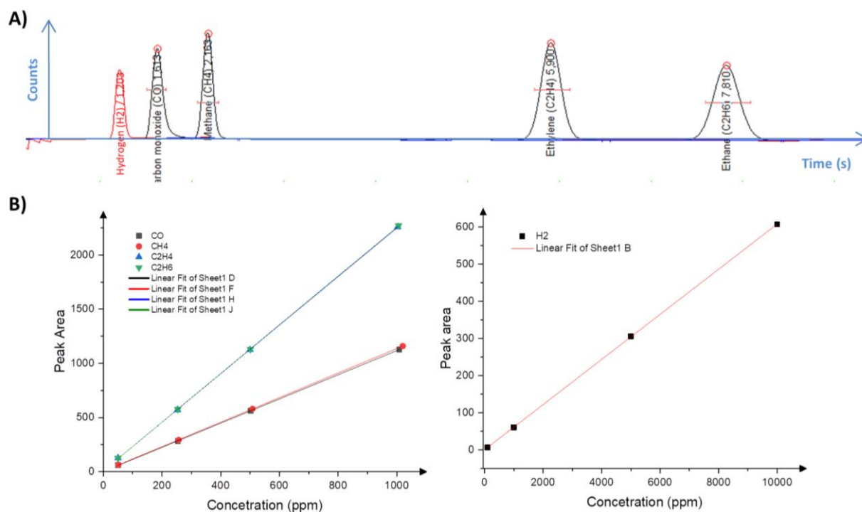
Figure S14. A) FID chromatogram with overlaid TCD signal for H_2 detection (red curve). The FID products elute in the following order: CO , CH_4 , C_2H_4 , and C_2H_6 . The good separation was achieved by optimizing the temperature of the column oven and carrier gas pressure. The shown example is for the mixture of 500 ppm ( CO , CH_4 , C_2H_4 , C_2H_6 ) and 5000 ppm of H_2 balanced in argon. B) Calibration curves for 4 points measurements are shown separately for FID (left) and TCD detected products (right).
