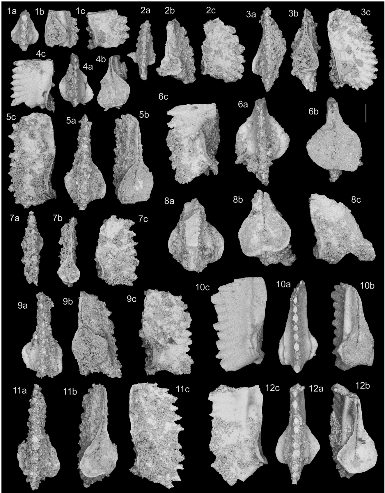
Fig. 6 - SEM images of conodonts from the Tulcea Veche locality, sample TV eastern base (GeoZS 6166).
