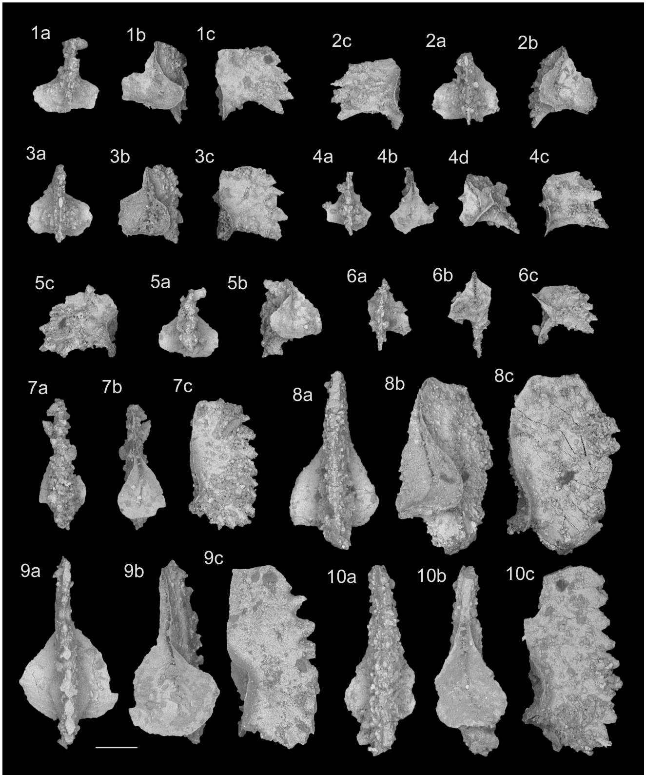
Fig. 7 - SEM images of conodonts from the Tulcea Veche locality, sample TV western base (GeoZS 6167). 1–3) Triassospathodus ex gr. hungaricus (Kozur & Mostler); 4) Triassospathodus hungaricus (Kozur & Mostler); 5–6) Triassospathodus sp.; 7–10) Triassospathodus symmetricus (Orchard).
