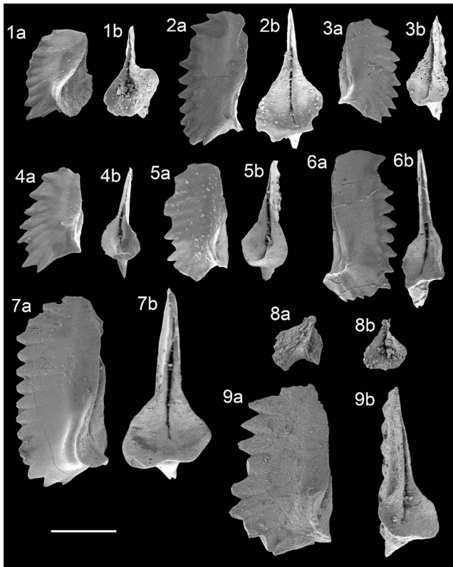
Fig. 5 - SEM images of conodonts from the Tulcea Veche locality. 1, 3–5, 9) Novispathodus abruptus (Orchard); 6) Triassospathodus ex gr. bomeri (Bender); 8) Novispathodus sp.; 2, 7) Triassospathodus symmetricus (Orchard). 1–5) sample GeoZS 4867; 6) sample GeoZS 4868; 7) sample GeoZS 4871; 8) sample GeoZS 4875; 9) sample GeoZS 4877. Scale bar: 200 microns; a) lateral, b) lower view.
