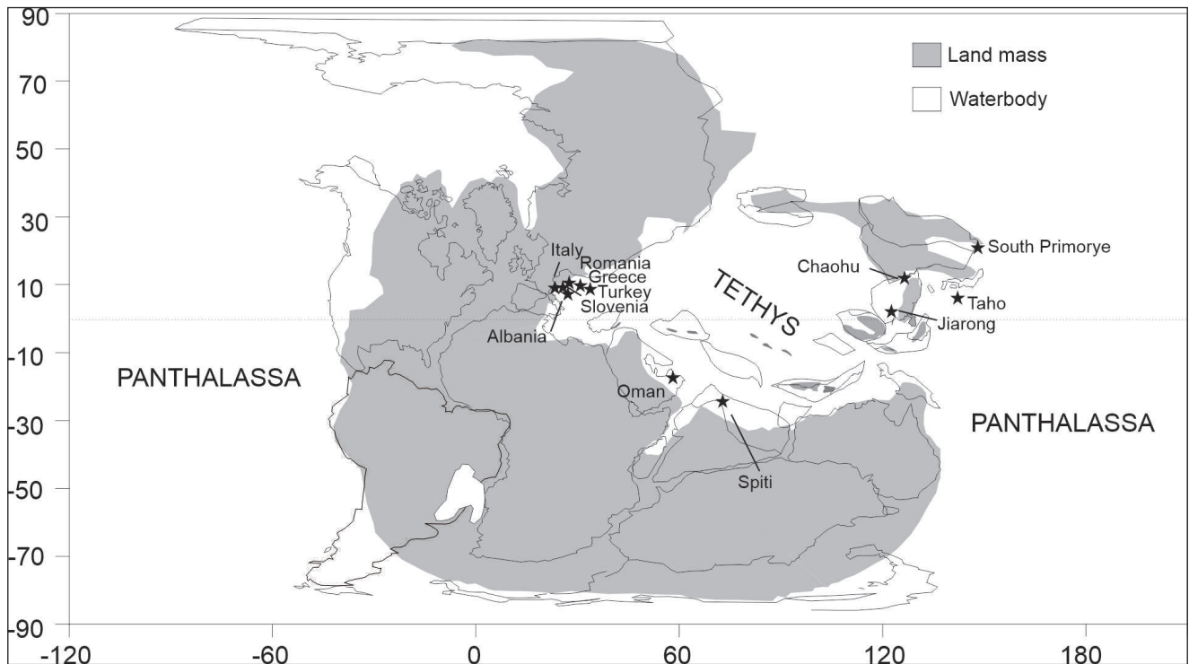
Fig. 4 - Paleogeography of the Olenekian world (modified after Péron et al. 2005). Asterisks indicate important localities mentioned in the text.
