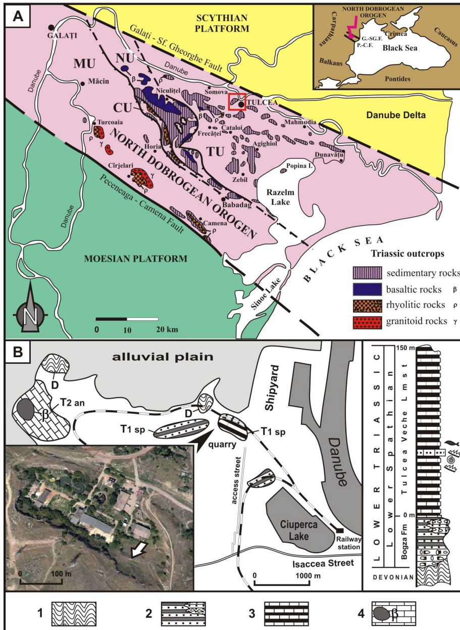
Fig. 1 - A) Geological sketch map of the Cimmerian North Dobrogean Orogen: MU – Măcin Unit; CU – Consul Unit; NU – Niculițel Unit; TU – Tulcea Unit. Inset map shows the location of the North Dobrogean Orogen (after Grădinaru 2000, modified). The box shows the studied locality. B) Geological map and the stratigraphic column of the Tulcea Veche (Old Tulcea) Promontory. 1 – Devonian (D); 2 & 3 – Lower Spathian ( T_{1sp} ), terrigenous sequence (2), limestone and marly shale (3); 4 – Middle Triassic, Anisian ( T_{2an} ), massive limestone with basalt intrusion ( \beta ). Inset Google Earth image of the Tulcea Veche Quarry, with the arrow showing the sequence sampled for conodonts.
