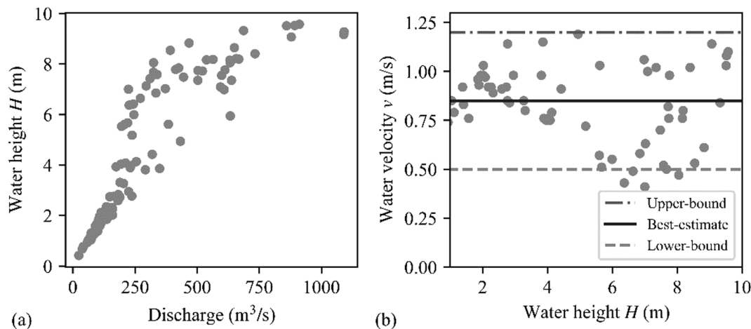
Fig. 3. Daily-max relations for numerical simulation of three flood events for years 2005, 2014 and 2015 – (a) Relationship between discharge and water height, (b) Relationship between water height and velocity, and three idealized scenarios.
