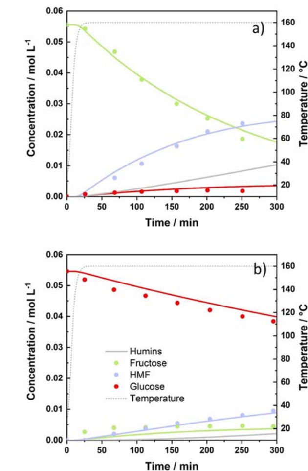
Fig. 5 Product distribution as a function of the time for (a) fructose and (b) glucose dehydration reaction in aqueous media without H-BEA at 160 °C, where symbols represent experimental points and lines corresponds to model values ● fructose, ● 5-HMF, ● glucose, – humins, ---- temperature.
