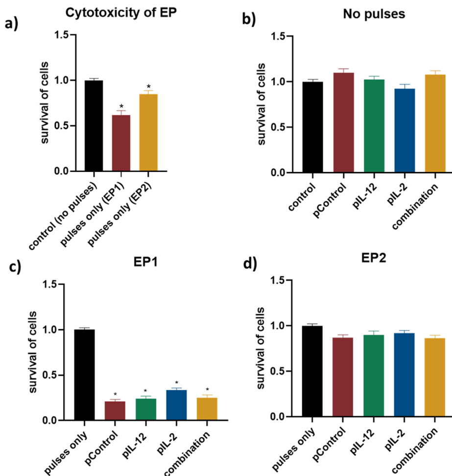
Fig. 2. Impact of the two electroporation protocols on the survival of B16.F10 cells without the plasmid addition (a). *p < 0.05 compared to the control and EP1 or EP2. In vitro cytotoxicity after plasmid addition coupled with two different electroporation protocols (c, d) and without electroporation (b) in B16.F10 cells. The results are shown as cell survival normalized to the pertinent control group (electroporated and nonelectroporated, without plasmid addition). The experiments were performed in 3 biological replicates, each consisting of 8 technical parallels. *p < 0.05 compared to pulses only. The values are expressed as the AM ± SEM.
