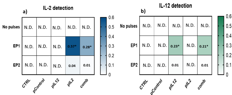
Fig. 3. In vitro mouse IL-2 (a) and IL-12 (b) mRNA expression after electroporation. a) Detection of IL-2 transcripts. b) Detection of IL-12 transcripts. The data are plotted as ΔCt (relative to the average of the two housekeeping Actb and Gapdh genes). The experiments were performed in 3 biological replicates, each consisting of 2 technical parallels. *p < 0.05 compared to EP1 or EP2. N.D. = not detected. The values are expressed as the AM ± SEM.
