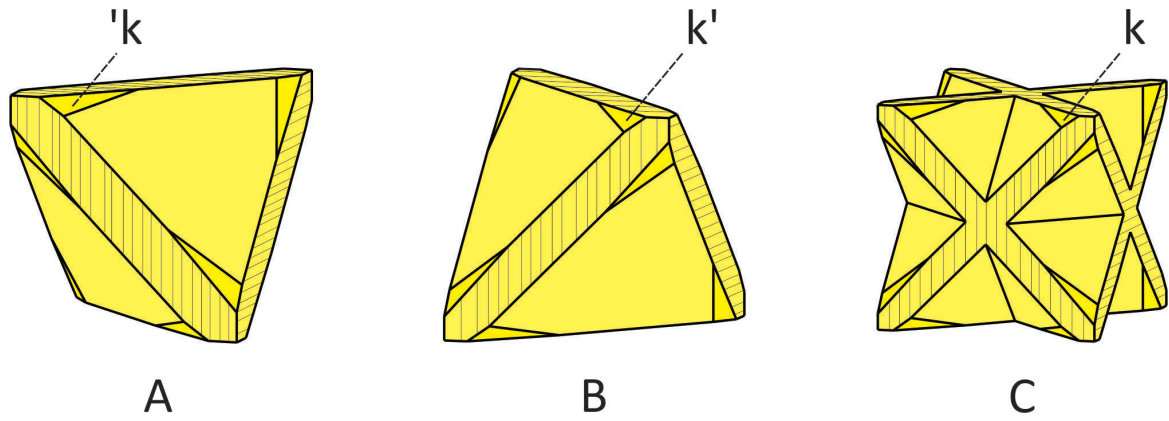
Fig. 6. (001)-interpenetration of single left- (A) and right-handed (B) tetrahedral crystals yields a twin (C). Chiral faces of tetrahedral pentagon dodecahedron forms 'k and k' transform to non-chiral dyakis-dodecahedron k (C).
