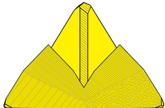
Fig. 8. (111)-interpenetration twins are never theoretically developed. Real crystals exhibit lower 3-fold symmetry, because of the incomplete development of the crystal that surrounds the central one. Drawings above and below show the projection of the right-handed twin along its [111]-twin axis and its projection perpendicularly to the same axis, respectively. Cube a faces are present only on the central crystal. Note the characteristic chiral-specific patterns.
