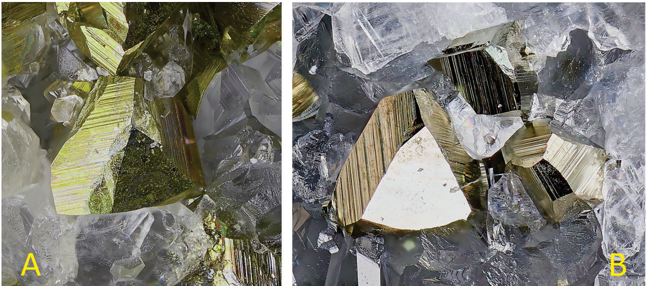
Fig. 4. Single pyrite crystals of the first generation on quartz matrix. Calcite crystallized later. Pyrite morphology is defined by tetrahedron t and striated cube a faces. Photographs A and B show left-handed and right-handed crystal, respectively. Note the class-specific faces of the corresponding left ' k\{11.10.14\} ' and right ' k\{\bar{1}.10.14\} ' tetrahedral pentagon dodecahedron. Both crystals measure one mm on their edges.
