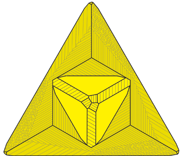
Fig. 7. 6-fold (111)-interpenetration twin (C) is a combination of two left- (shown in the drawing) or two right-handed tetrahedral single crystals, whereby one of them is simultaneously rotated by 60° (B) with respect to the other one (A).
