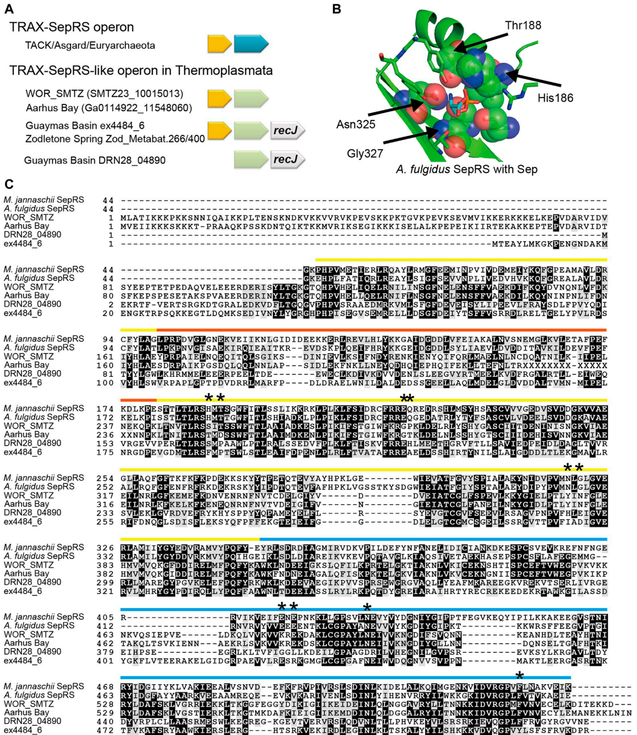
FIGURE 6 | Characterization of SepRS-like proteins from two lineages of Thermoplasmata archaea (A) The operon structures of the four SepRS-like genes identified. Like many SepRS genes, three SepRS-like genes are headed by a TRAX homolog gene. In the Guaymas Basin hydrothermal vent lineage and the Zodlone Spring lineage, the SepRS-like genes are followed by a predicted recJ gene (B) The four residues important for Sep recognition by SepRS are altered in SepRS-like proteins (C) Multiple sequence alignment of SepRS-like proteins with two reference SepRS proteins. Interesting mutations are denoted by stars. The color bars represent the domain structure and follow the same scheme as in Figure 3, with the yellow bar denoting the catalytic domain, the orange bar denoting the inserted domain, and the blue bar denoting the anticodon binding domain. A part of the Aarhus Bay SepRS-like sequence remains elusive (indicated with Xs).
