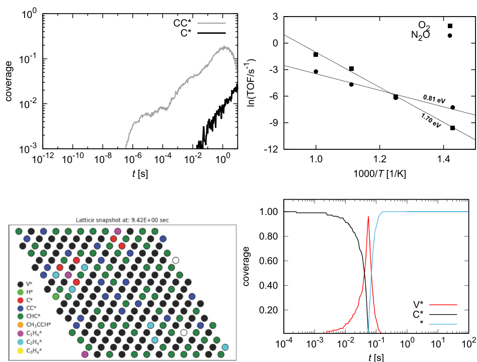
Figure 13. (Top left) Coverage of the catalyst with transient CC^* and C^* at T = 900 K and p_{C_3H_8} = p_{O_2} = 1 bar; (top right) the Arrhenius plot for the deactivation of the oxidized catalyst (measured as the buildup of CC^* and C^* ) when using different oxidants ( O_2 and N_2O ); (bottom left) lattice snapshot after 9.42 s; (bottom right) regeneration of the coked catalyst with 1 bar O_2 at 900 K when the C_3H_8 feed is cut off.
