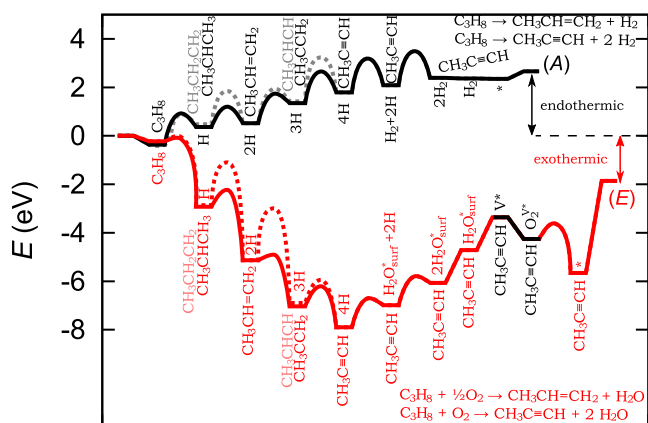
Figure 5. Potential energy surface for propane dehydrogenation over reduced (A) and oxidized (E) \text{Cr}_2\text{O}_3(0001) . Deep dehydrogenations are not shown. Upon the removal of surface oxygen as \text{H}_2\text{O} , the oxidized surface is reduced and reoxidized with \text{O}_2 or \text{N}_2\text{O} (latter not shown). Intermediates in light color and transition states connected with dashed lines are energetically disfavored.
