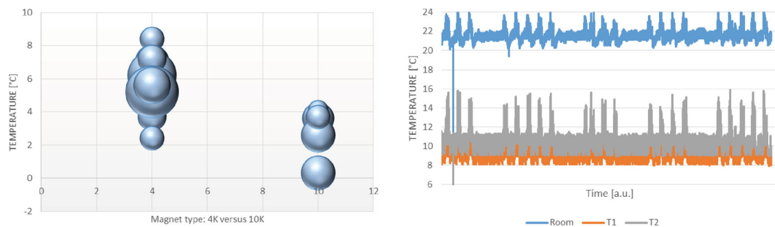
Figure 13. Temperature distribution and classification (left) and temperature correlations (right).
