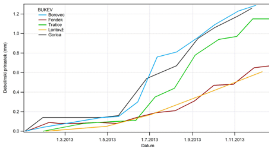
Graf 1: Letni debelinski prirastek bukke na petih ploskvah intenzivnega spremljanja stanja gozdnih ekosistemov – Trnovski gozd (Fondek), Kočevska Reka (Borovec), Zasavje (Lontovž), Pohorje (Traticice) in Loški Potok (Gorica) v letu 2013 // Graph 1: Annual radial increment of beech trees on five intensive forest monitoring plots – Trnovski gozd (Fondek), Kočevska Reka (Borovec), Zasavje (Lontovž), Pohorje (Traticice) and Loški Potok (Gorica) in 2013
