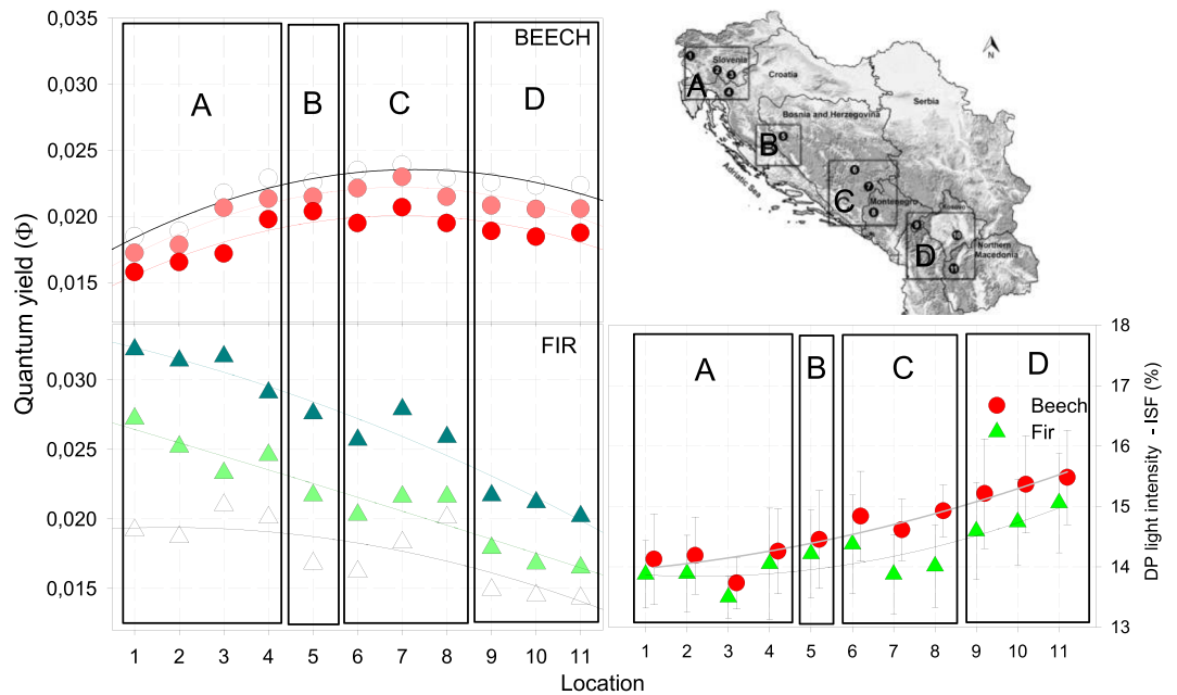
Figure 8. Physiologic and morphologic responses within growth areas (A–D) along the studied gradient.
